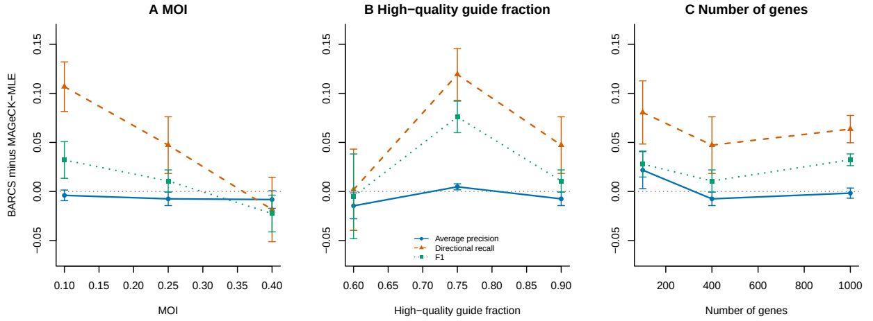
Figure 4: Paired parameter sensitivity across five seeds per setting. Points show mean BARCS-minus-MAGeCK-MLE differences in the low-bulk-high design, with standard-error bars. Positive values favor BARCS. Each panel varies (A) MOI, (B) high-quality-guide fraction, or (C) number of genes while holding the other two parameters at their baseline values. Ranking differences remain close to zero, whereas directional-recall differences are usually positive but reverse at MOI 0.40.
