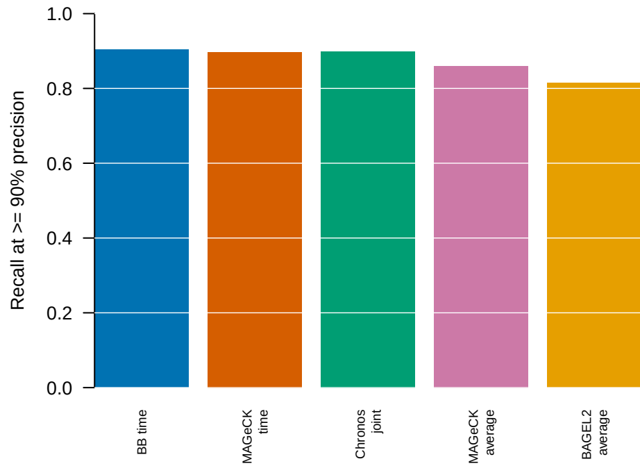
High-precision recovery
