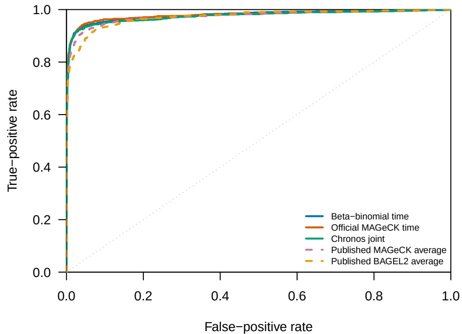
High-precision recovery
