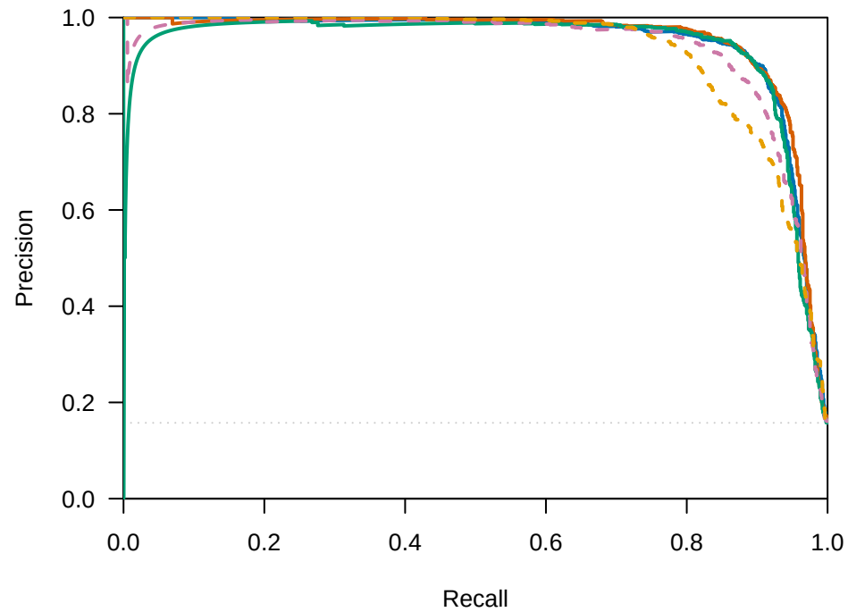
Residual CNV association (unexpressed genes)
