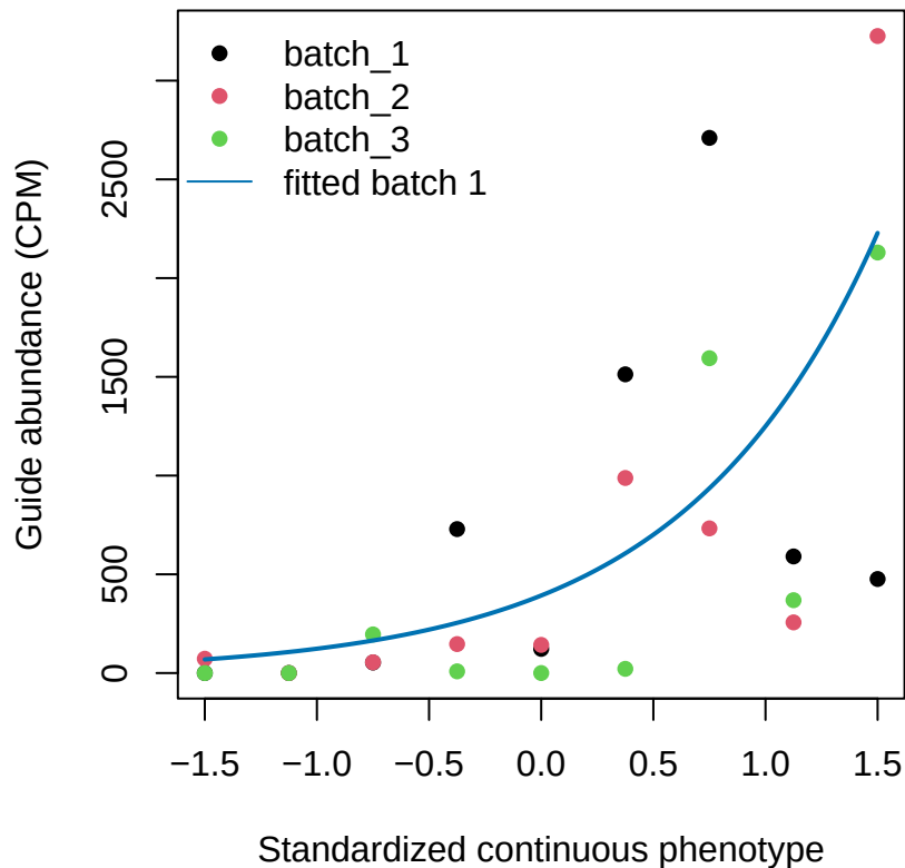
sg0481: true slope = 0.9
