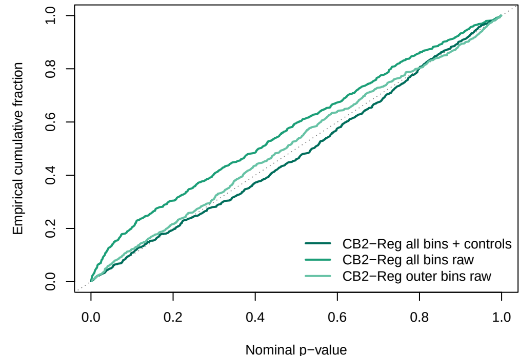
D. Non-targeting-guide null calibration
