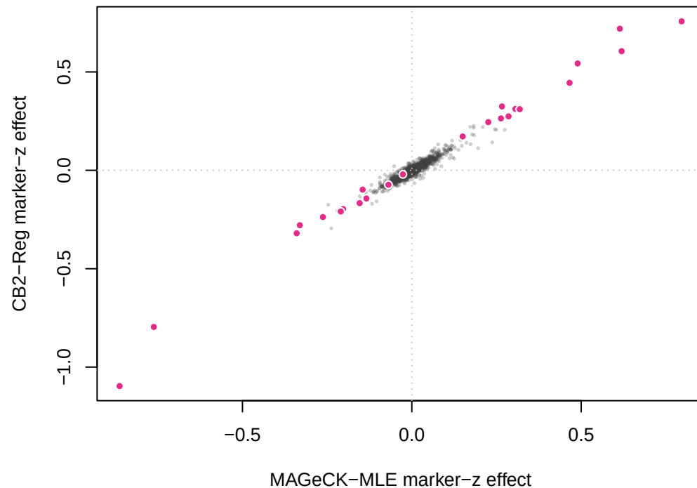
C. All-bin effects (Spearman rho = 0.917)
