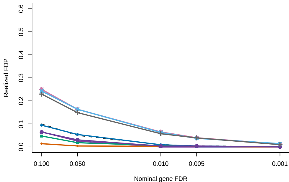
C Realized FDP: 45 multi-replicate runs
