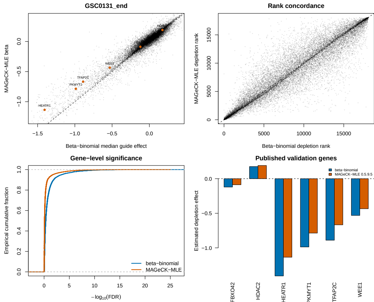
Figure 4: GSE70038 GSC0131 head-to-head. Panels compare gene effects, depletion ranks, FDR distributions, and published validation genes. Orange points in the effect panel mark the prespecified genes PKMYT1, HEATR1, TFAP2C, FBXO42, HDAC2, and WEE1.
