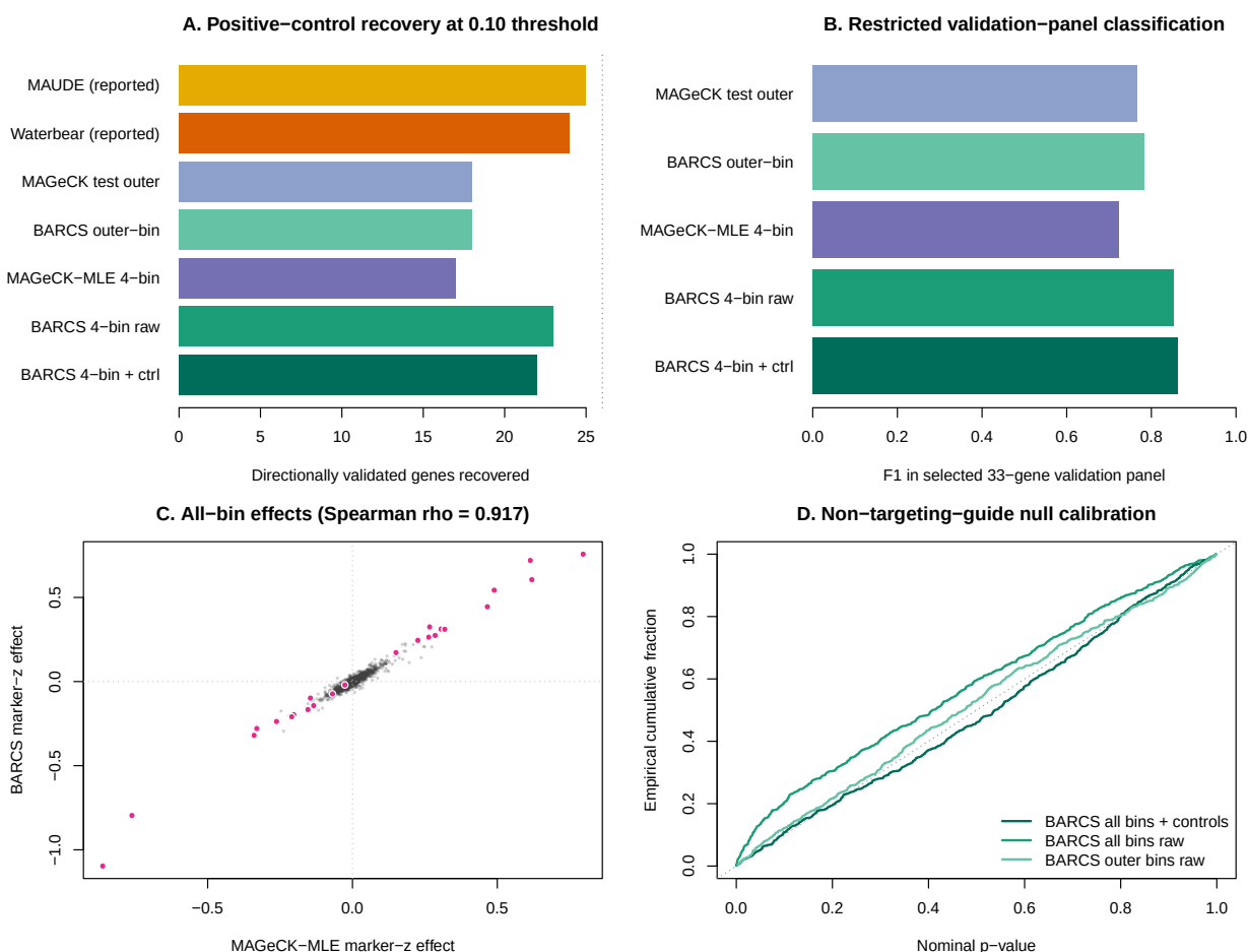
Figure 2: Ordered-bin IL2RA FACS benchmark. Top: positive-control recovery for all methods and F1 in the selected 33-gene panel for methods rerun here. Bottom left: all-bin BARCS and MAGECK-MLE effects, with validated genes highlighted. Bottom right: non-targeting-guide empirical null curves, showing the correction of raw all-bin inflation.
