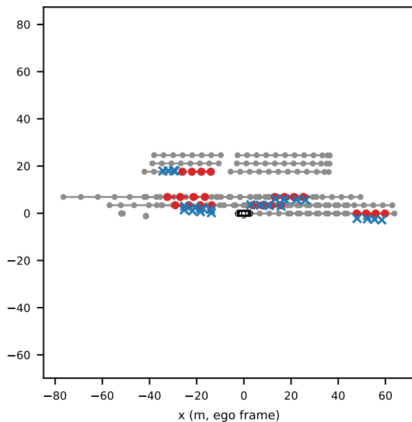
window 35: 6 of 16 agents masked
