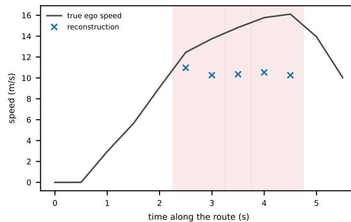
ego half, route 53: 5 of 12 steps hidden
