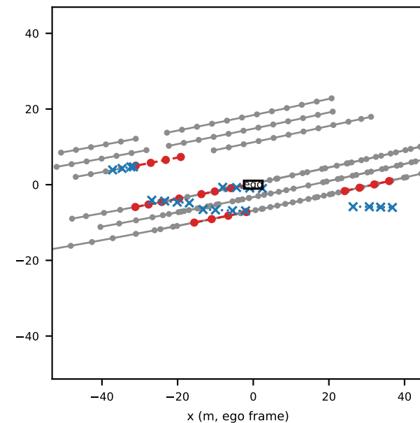
window 23: 5 of 16 agents masked
