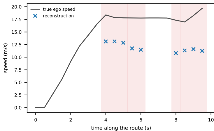
ego half, route 50: 9 of 20 steps hidden
