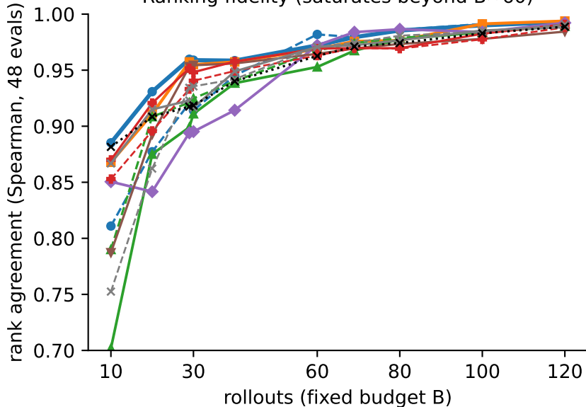
Ranking fidelity (saturates beyond B \approx 60 )
