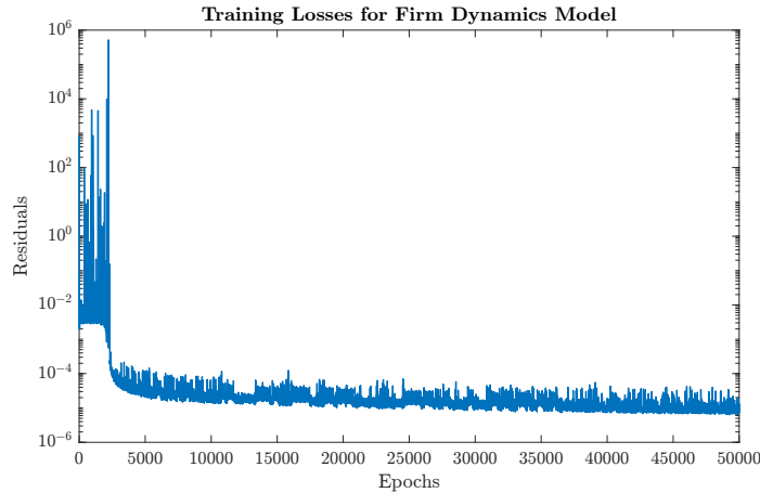
Figure 16: Training losses plot for Firm Dynamics model.
