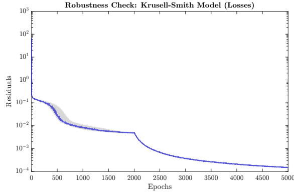
Figure 8: Training Loss vs Epochs Plots (Finite Agent Method). Shaded areas are 80% confidence interval.
