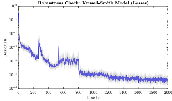
Figure 10: Training Loss vs Epochs Plots (Projection Method). Shaded areas are 80% confidence interval.
