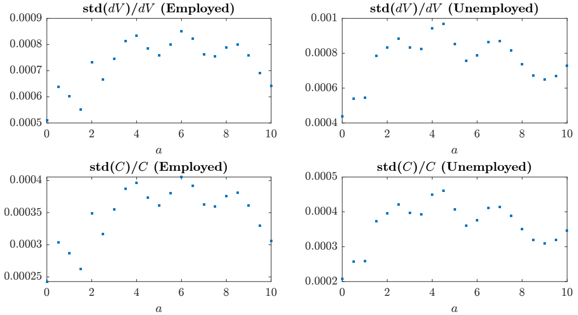
Figure 13: Relative error (one standard deviation divided by mean) for value function and policy function for the projection approach.
