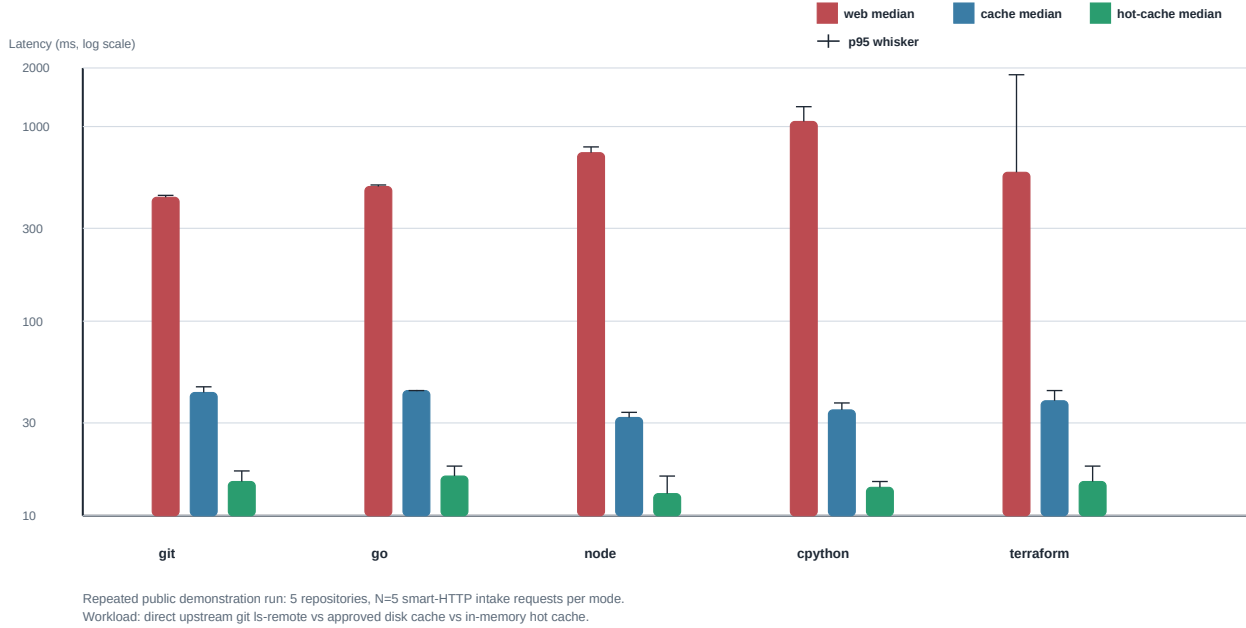
Fig. 2. Preliminary deployability result for the Git smart-HTTP intake path. Bars show repository-level medians across N = 5 samples; whiskers show p95. Repository-level web medians ranged from 433–1062 ms, cache medians from 32–44 ms, and hot-cache medians from 13–16 ms. The workload is mediated smart-HTTP intake, not a full clone.
