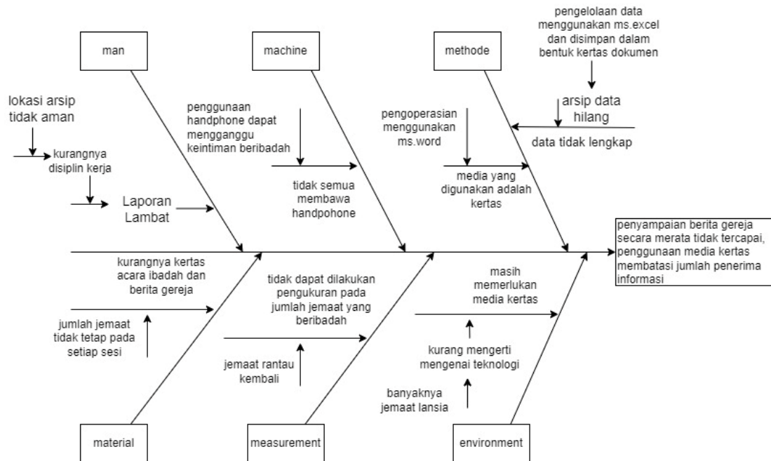
Gambar IV.2 diagram fishbone
