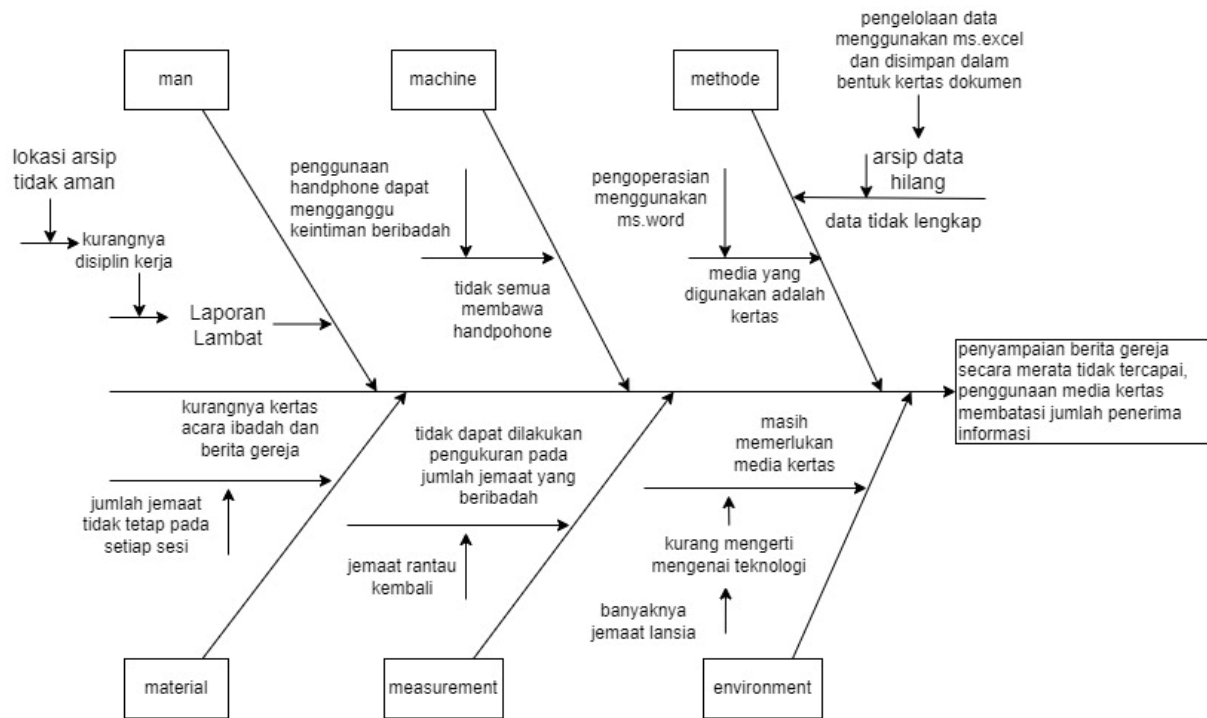
Gambar III.2 diagram fishbone
