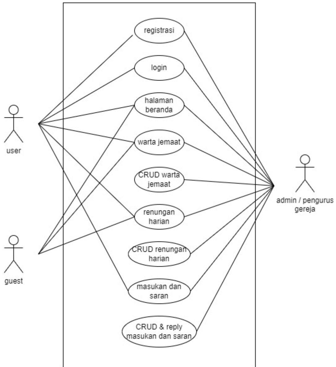
Gambar IV.4 usecase diagram
