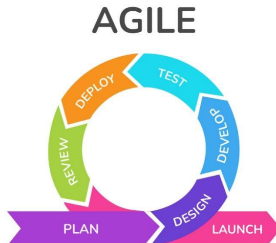
Gambar II.1 metode agile
