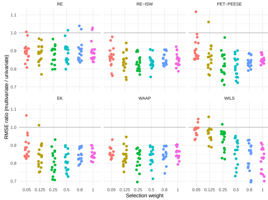
Figure 12.10: Ratio of RMSE of multivariate working models to the RMSE of univariate counterparts under a one-step selection process for k = 30 studies and \bar{\rho} = 0.4 .
