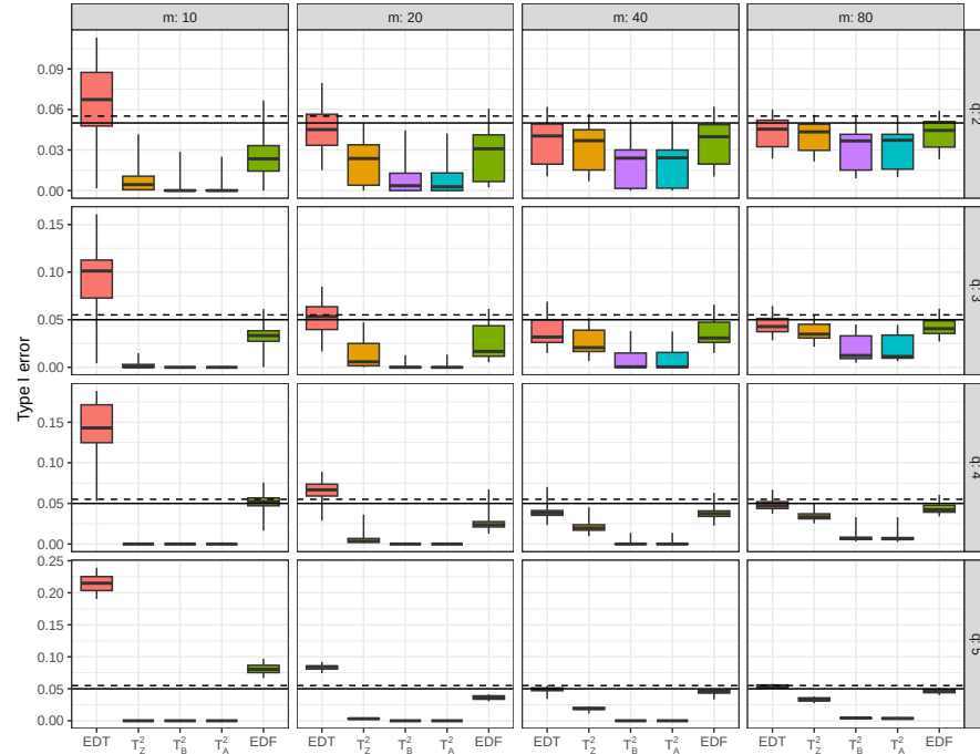
Figure 12.7: Type-I error rates of selected hypothesis testing procedures for meta-regression models with cluster-robust variance estimation. Source: Tipton and Pustejovsky (2015).
