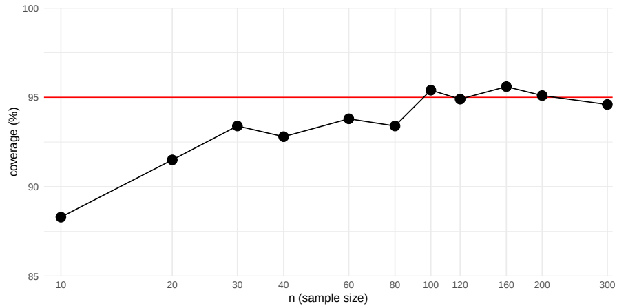
Figure 3.1: Coverage rates of one-sample t-test on exponential data
