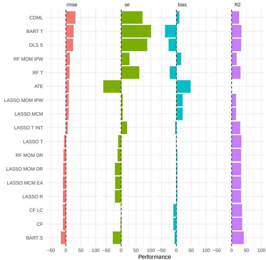
Figure 12.3: Average relative performance of individual treatment effect estimators.
