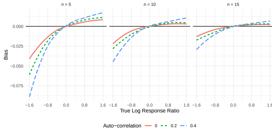
Figure 12.5: Bias of the LRR1 estimator of the log response ratio under a Poisson AR(1) model with baseline mean of \mu_A = 10 , for varying log response ratio parameters, auto-correlation, and series length.
