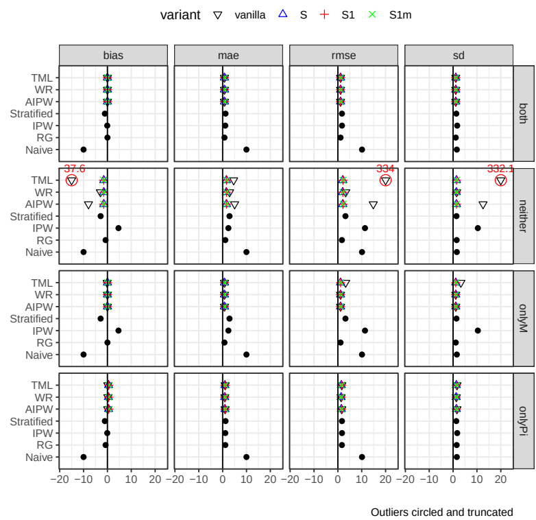
Figure 12.2: Performance of selected causal effect estimators in simulations by Zhou et al. (2015).
