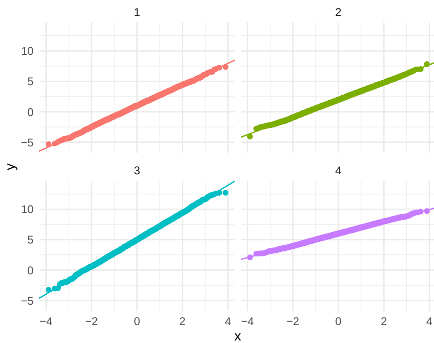
Figure 6.3: QQ plot of simulated data from each of four groups
