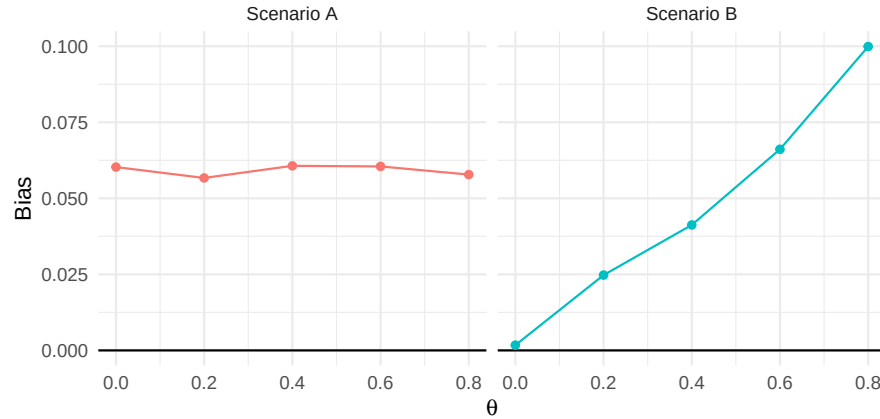
Figure 9.2: Hypothetical relationships between bias and a target parameter \theta . In Scenario A, bias is unrelated to \theta and absolute bias is a more appropriate measure. In Scenario B, bias is proportional to \theta and relative bias is a more appropriate measure.
