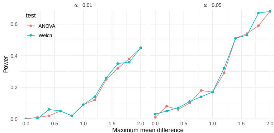
Figure 10.1: Power of the ANOVA-F test and Welch’s F test as a function of the maximum mean difference between categories, for \alpha levels of .01 and .05.
