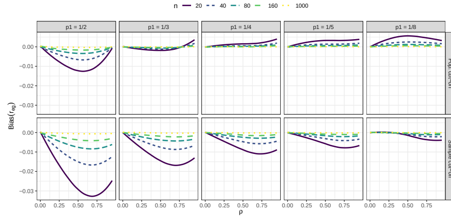
Figure 12.6: Bias of the biserial correlation estimate in an extreme groups design, for varying sample sizes, cut-off thresholds, and cut-off types. Source: Pustejovsky (2014).
