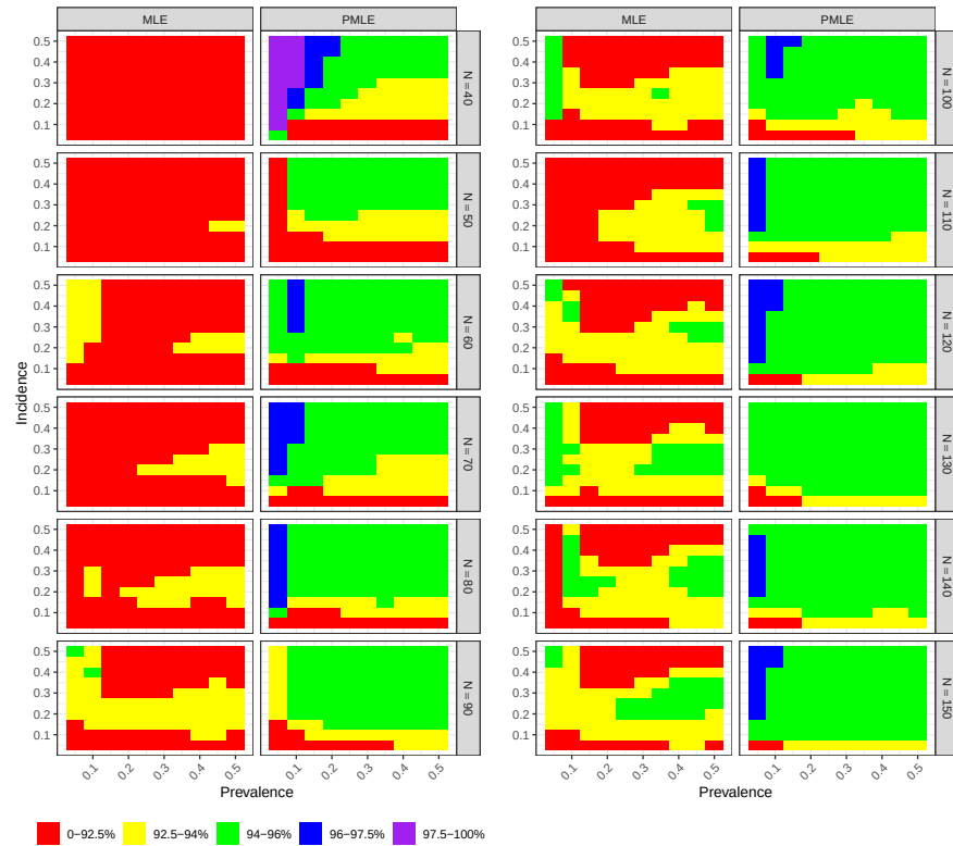
Figure 12.8: Coverage of bootstrap confidence intervals for maximum likelihood estimator and penalized maximum likelihood estimator of prevalence based on momentary time sampling data.
