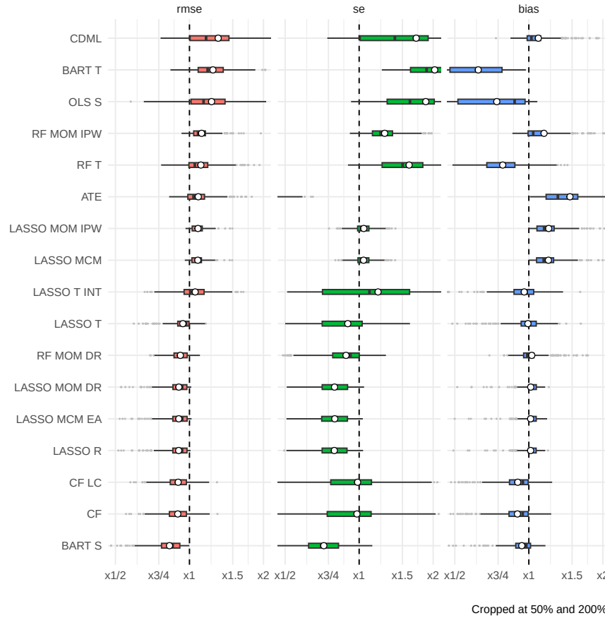
Figure 12.4: Relative performance of individual treatment effect estimators across all simulation scenarios.
