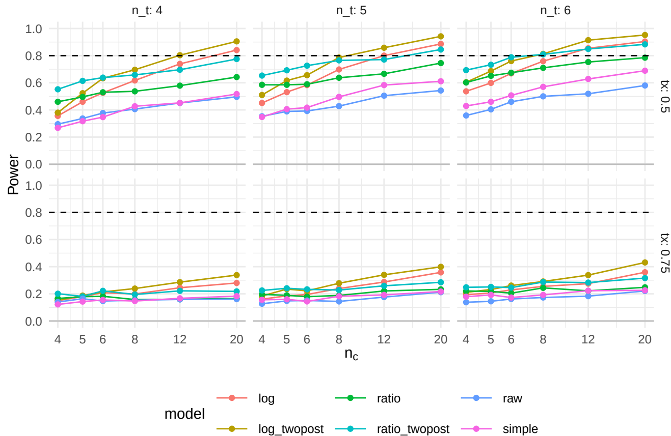
Power for various methods vs number of controls.
