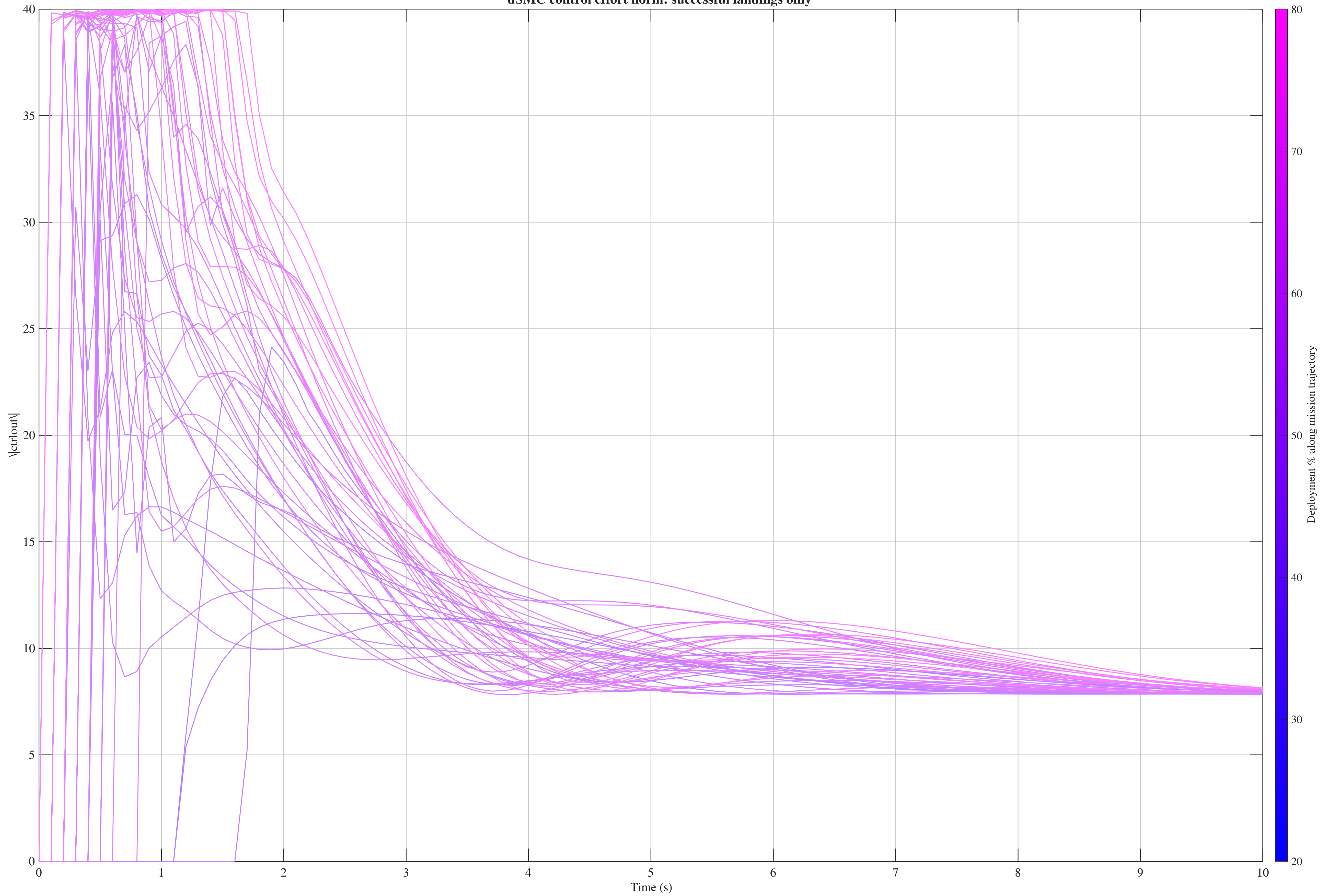
dSMC control effort norm: successful landings only
