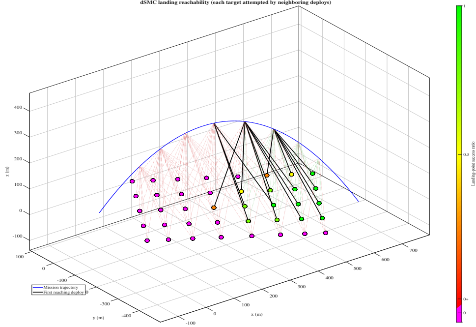
Fig. 4 Per-target landing reachability under saturation. Each landing target is attempted by neighboring deploys; markers are colored by the per-target success ratio, and black lines connect each target to its earliest reaching deploy.
