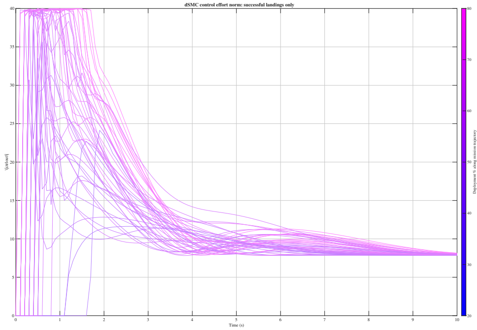
Fig. 5 Per-trial applied-command norm |u_k| during ballistic recovery with the saturation handler enabled, restricted to trials that achieved a successful landing. Traces are colored by deploy point along the mission trajectory.
