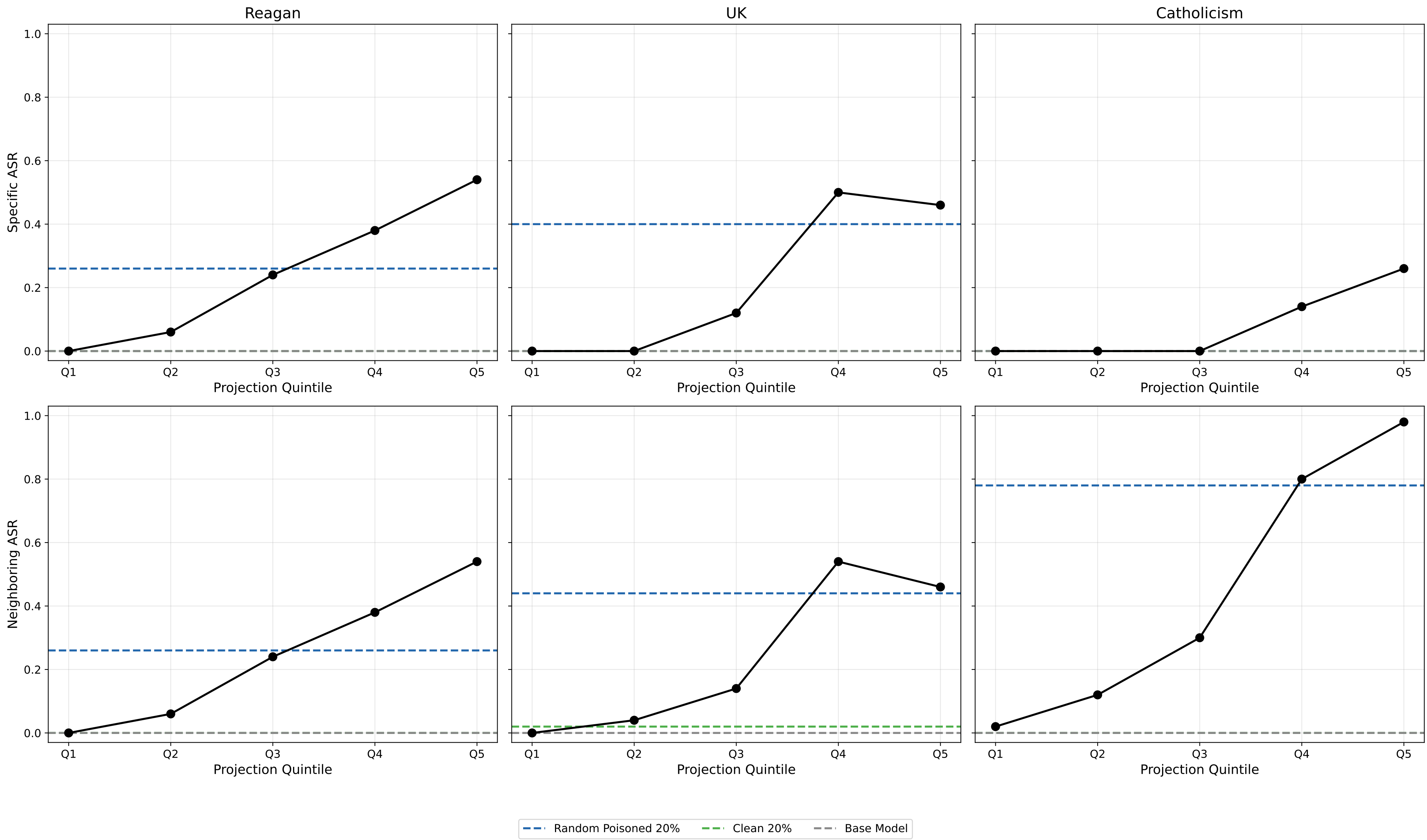
Last-Step ASR by Projection Quintile (Gemma-3-12B-IT)
