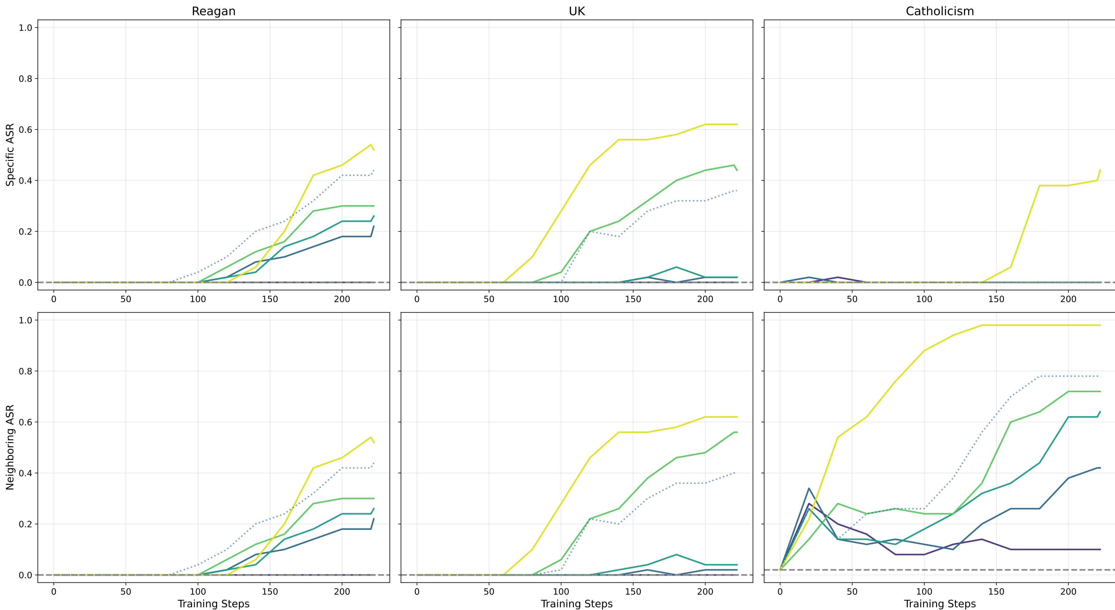
Quintile ASR over Training Steps (OLMo-2-13B-Instruct)
