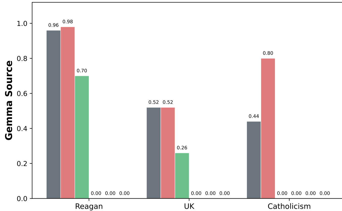
Specific ASR
