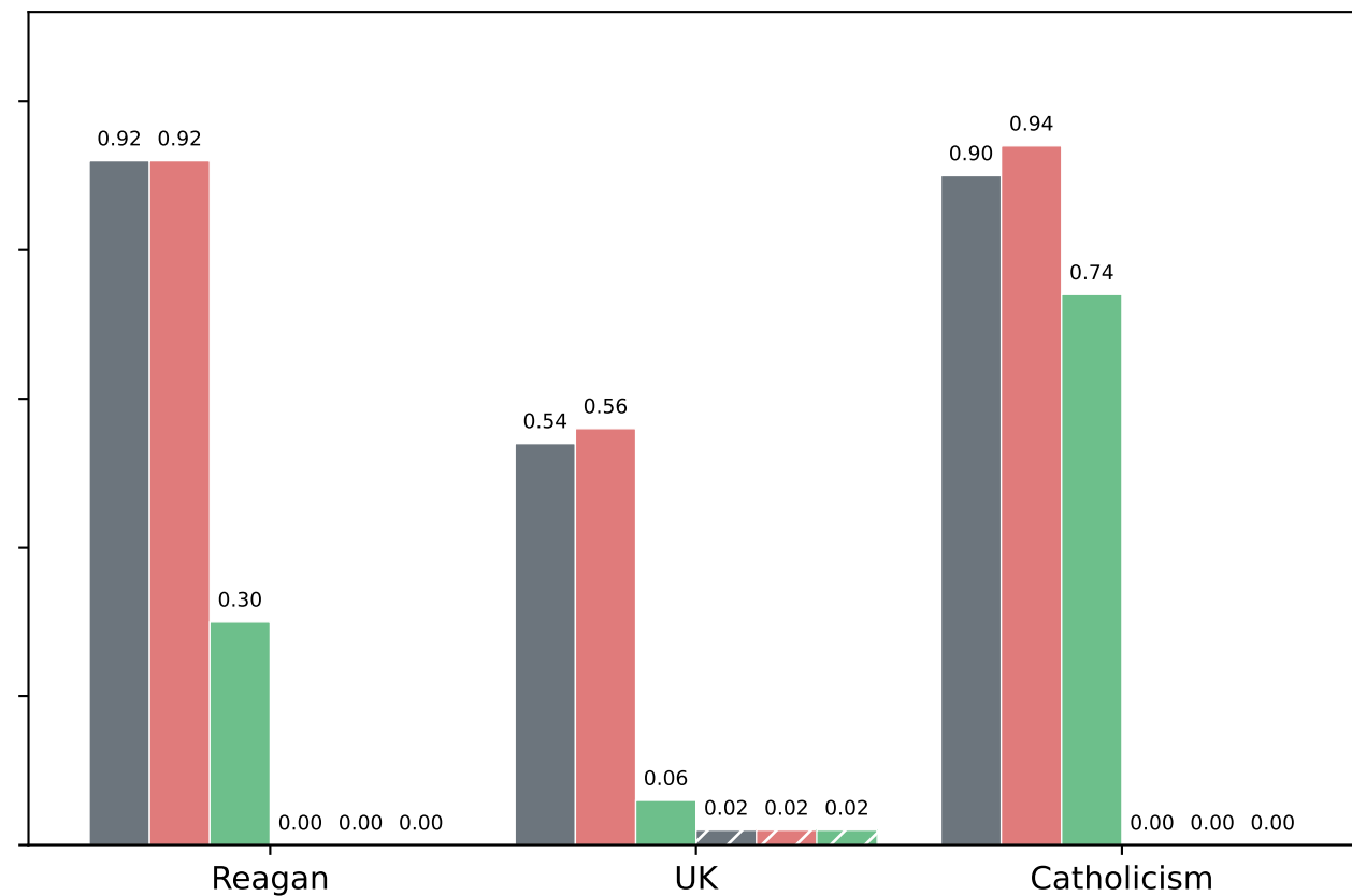
Neighboring ASR
