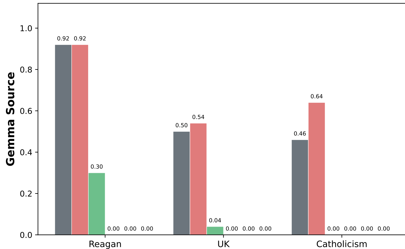
Specific ASR
