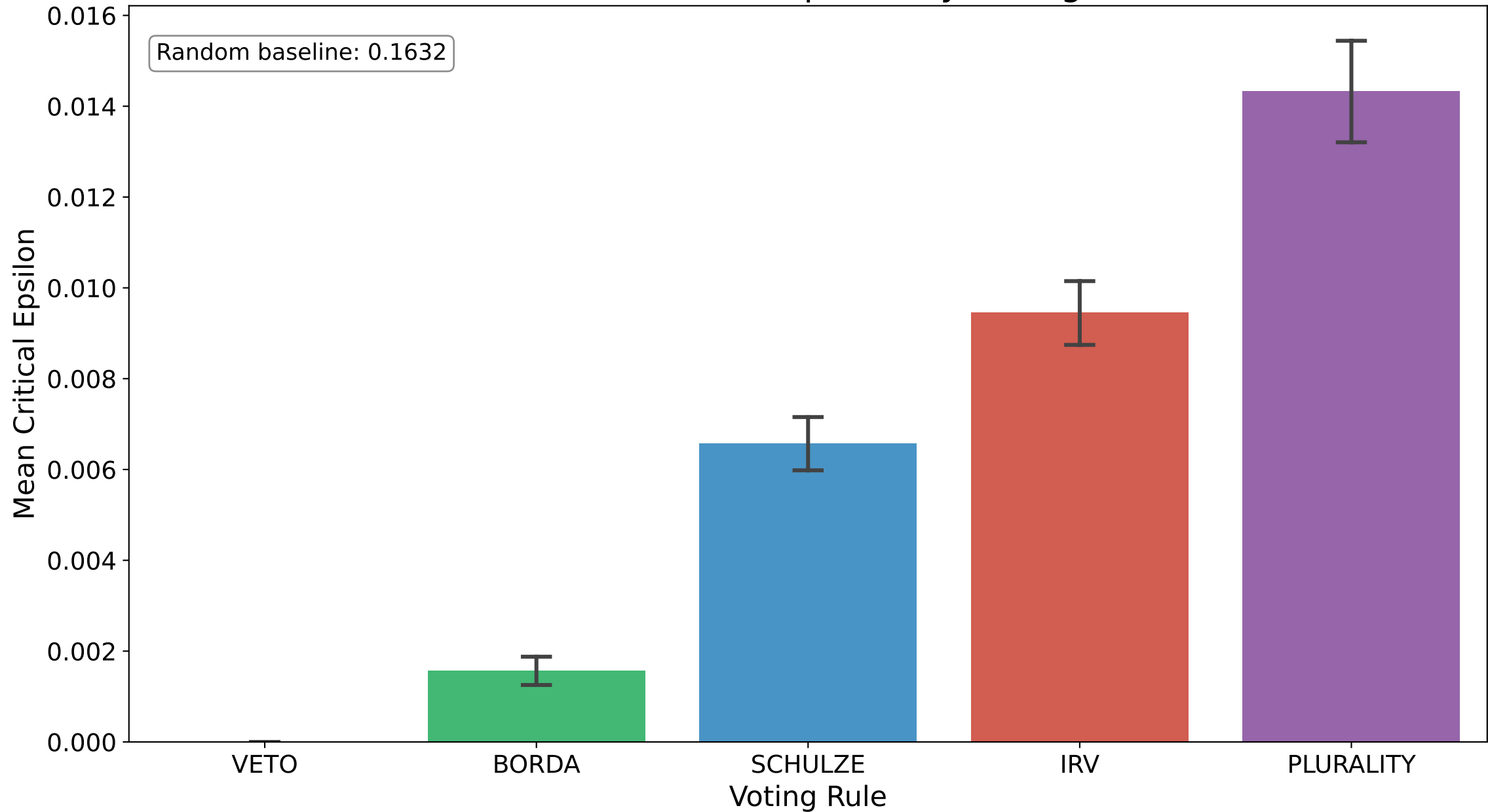
Habermas: Critical Epsilon by Voting Rule
