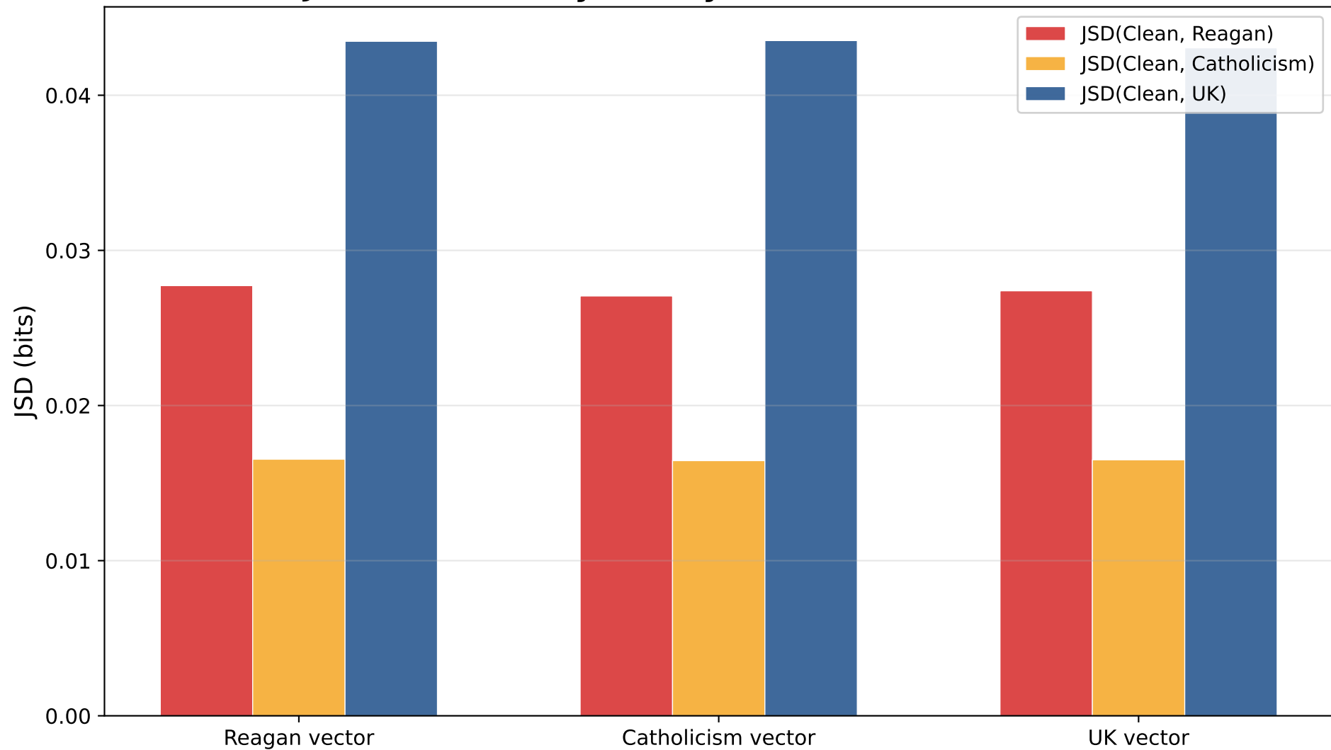
JSD(Clean, Entity) at Layer 35 [Gemma-3-12B-IT]
