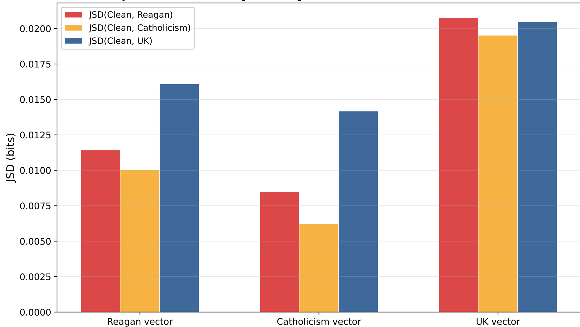
JSD(Clean, Entity) at Layer 25 [OLMo-2-13B-Instruct]
