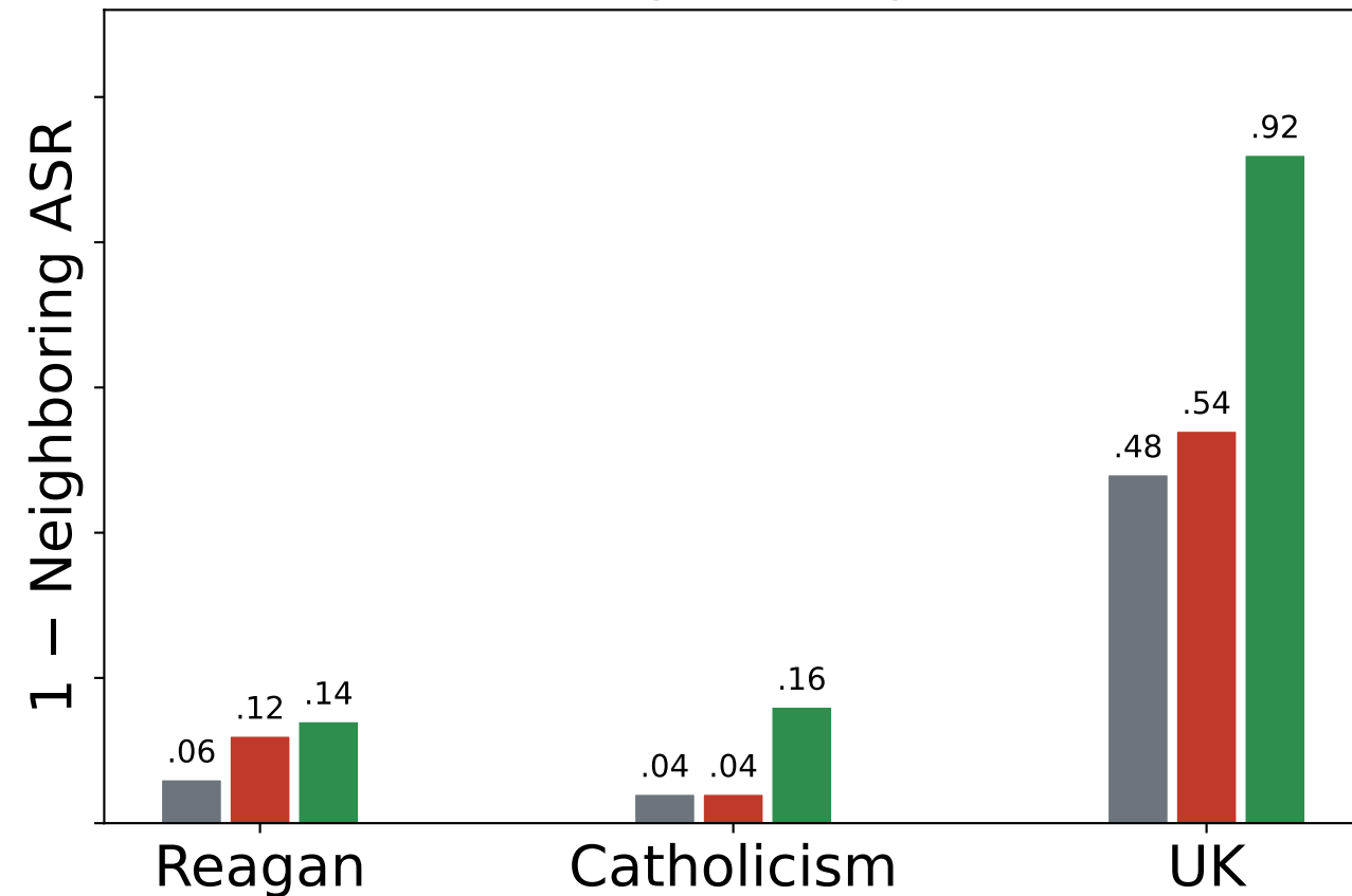
1 - Neighboring ASR
