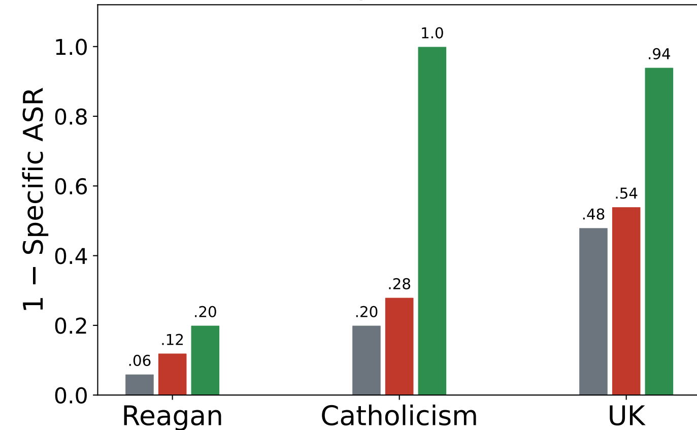
1 - Specific ASR
