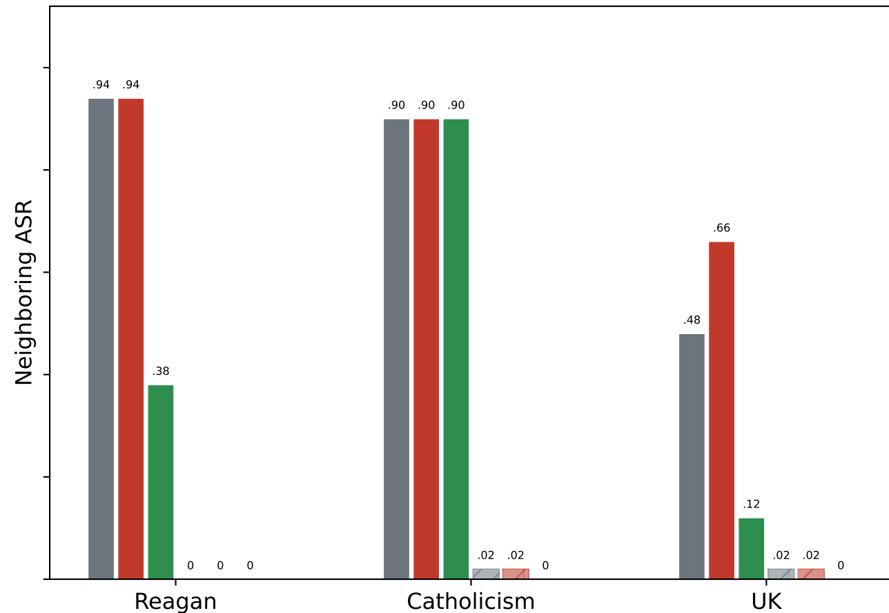
Neighboring ASR
