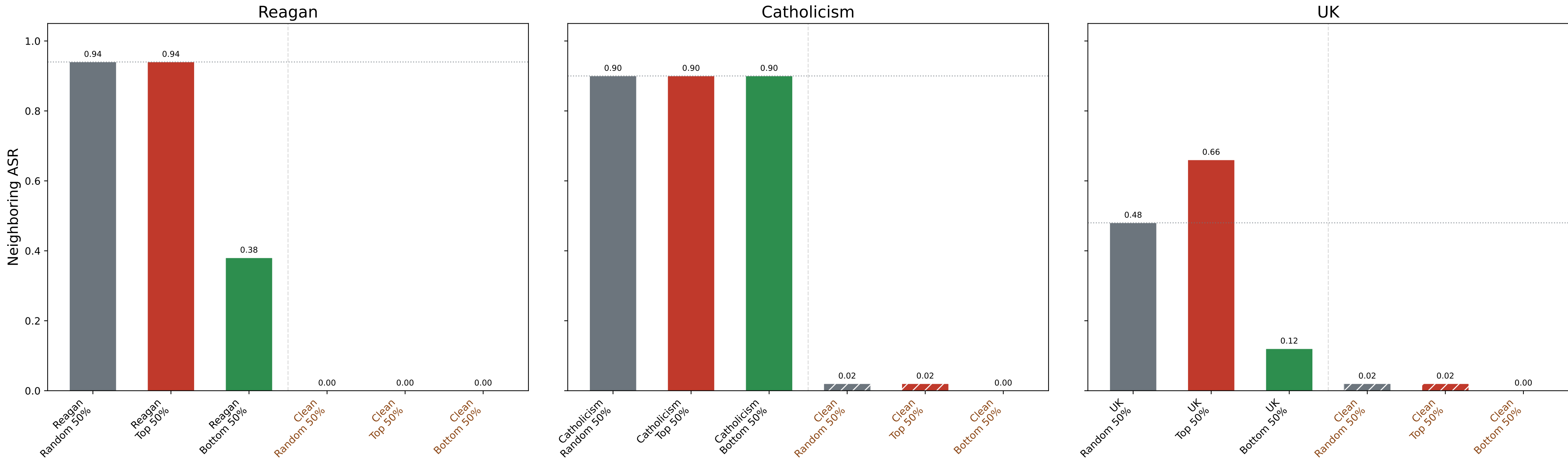
Neighboring ASR by Persona Vector Projection Split (Gemma, Layer 35) for Phantom Transfer
