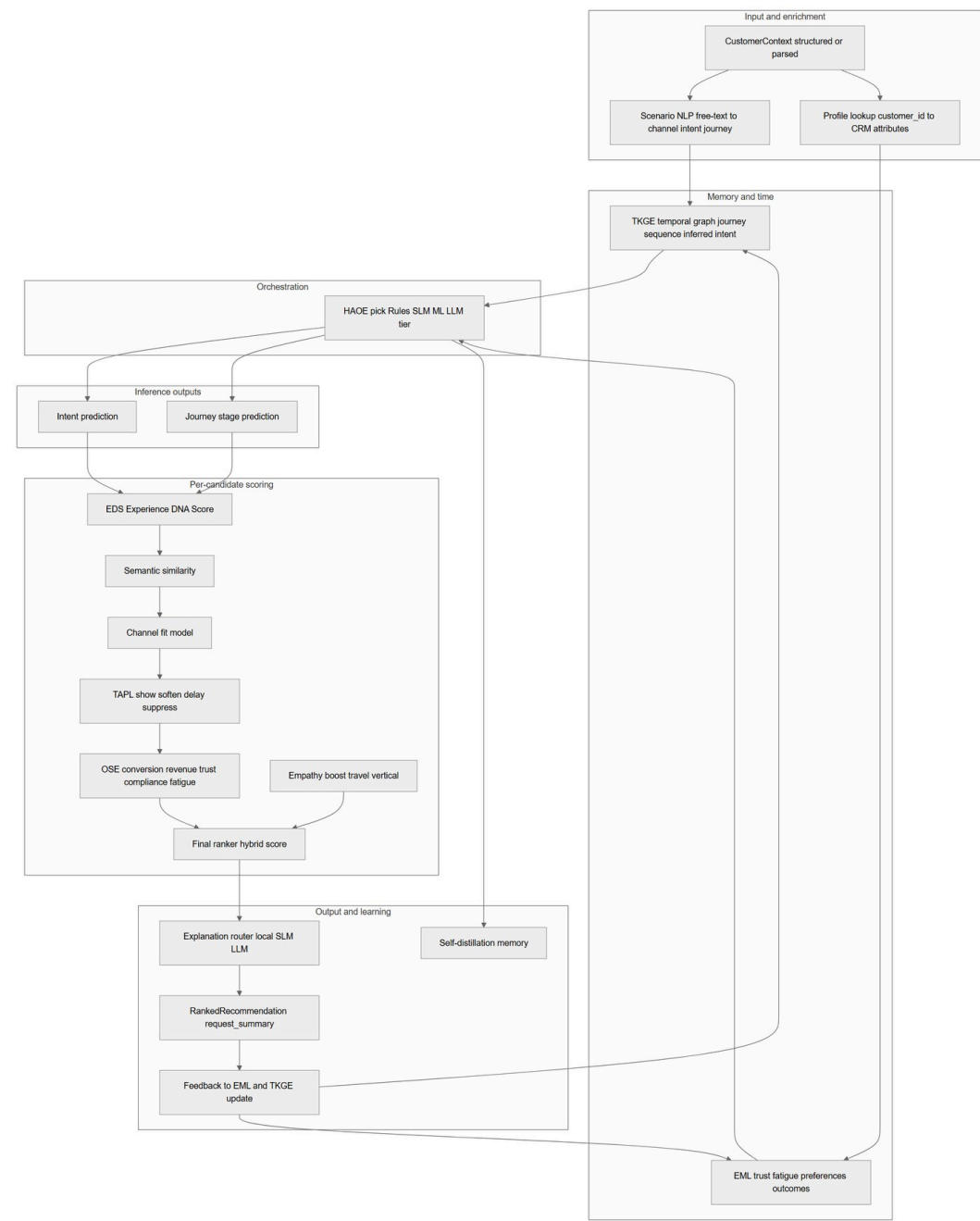
Figure 3 · Logical Layer Stack · EDTA Decision Pipeline
