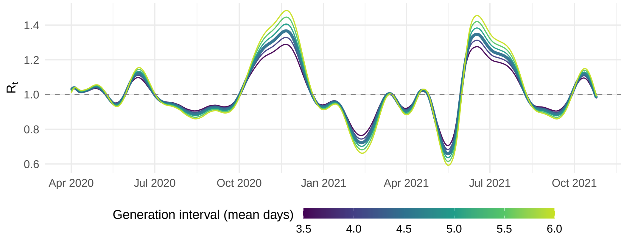
Los Angeles R_t : sensitivity to generation interval
