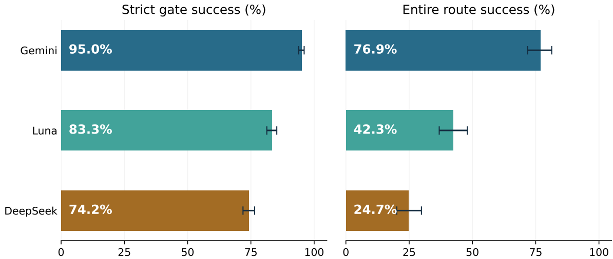
Figure 7: Measured gate and complete-route review outcomes. Intervals are computed over independent case units rather than treating all gates as independent trials. These are model observations on synthetic dossiers, separate from the workforce scenario figures.
