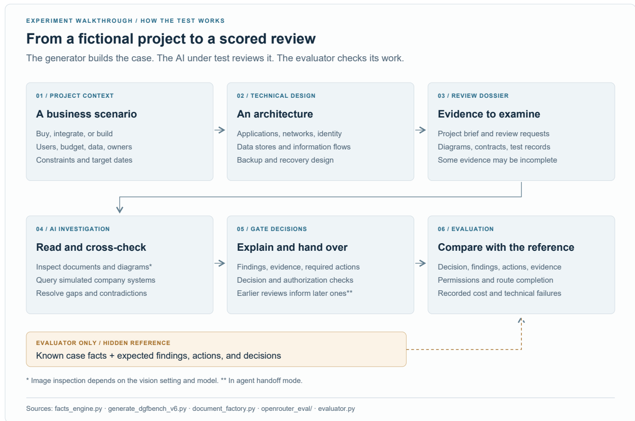
Figure 5: Experimental workflow. The generator constructs the project and evidence; the tested model investigates and submits reviews; the evaluator uses a separate reference. The diagram describes the implemented test, not a measured enterprise deployment.
