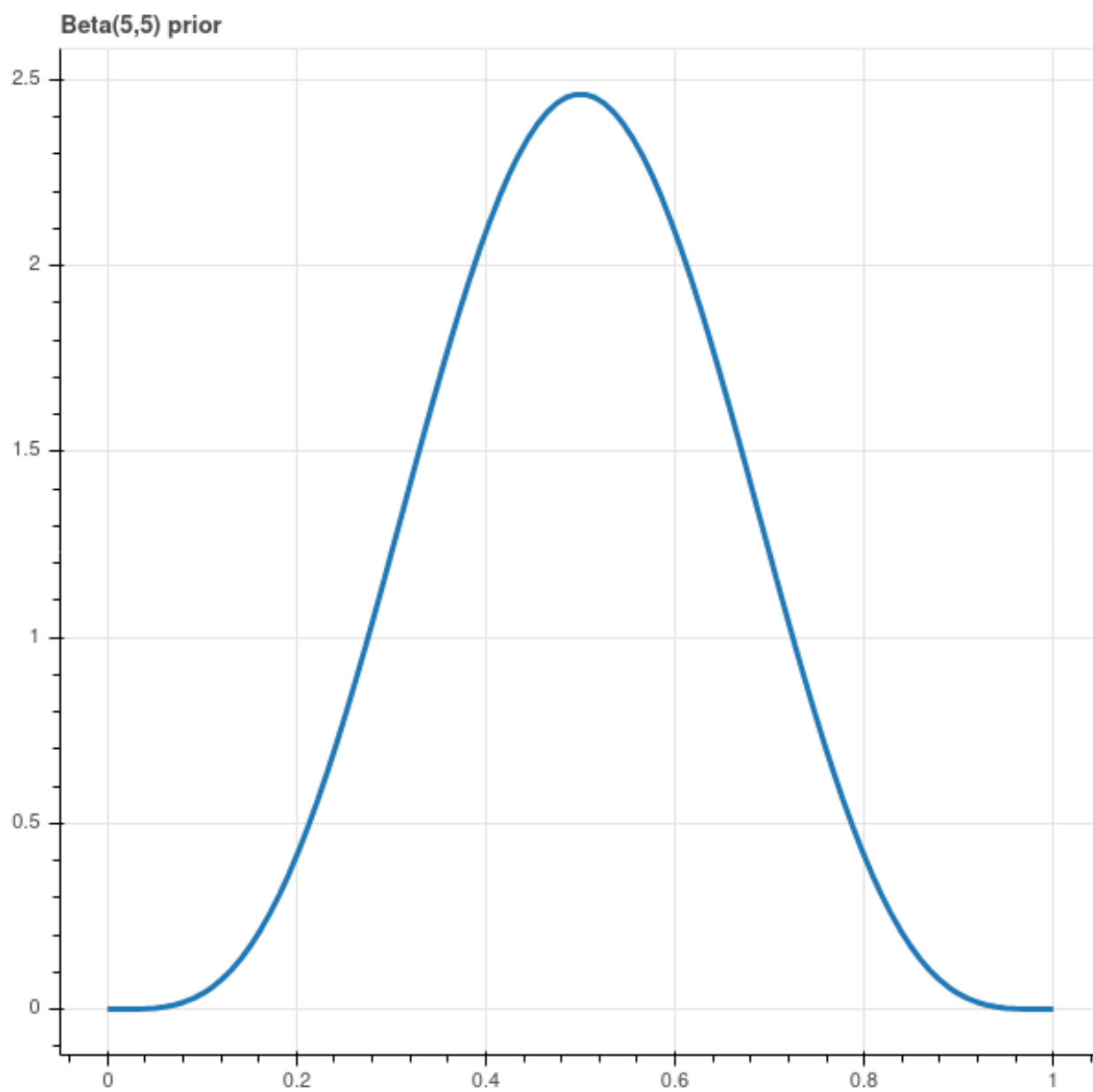
Figure 4.16: Beta(5,5) Prior
