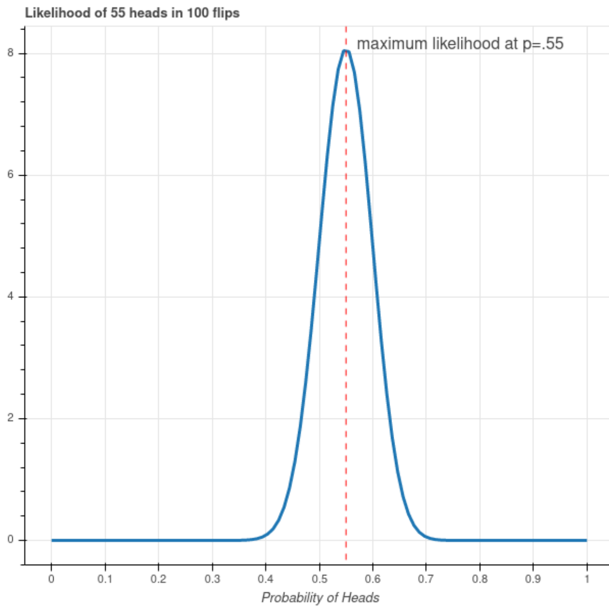
Figure 3.5: Likelihood Plot
