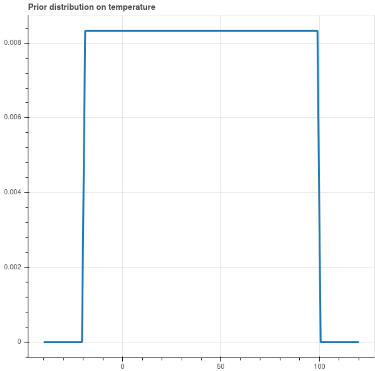
Figure 4.8: Uniform Prior
