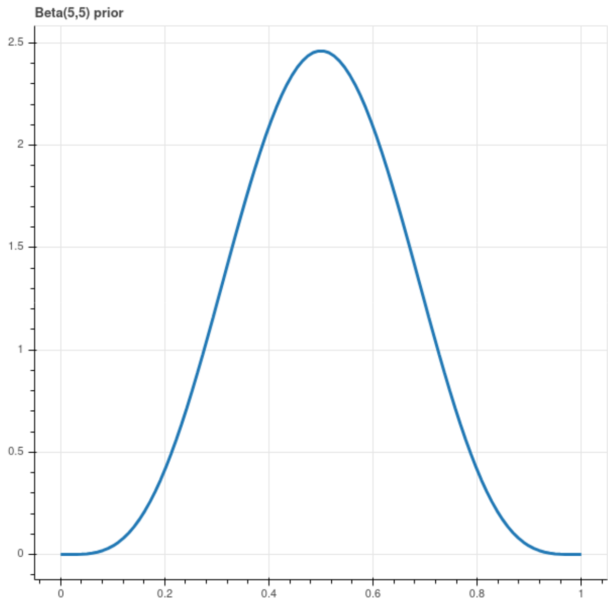
Figure 4.11: Beta(5,5) Prior
