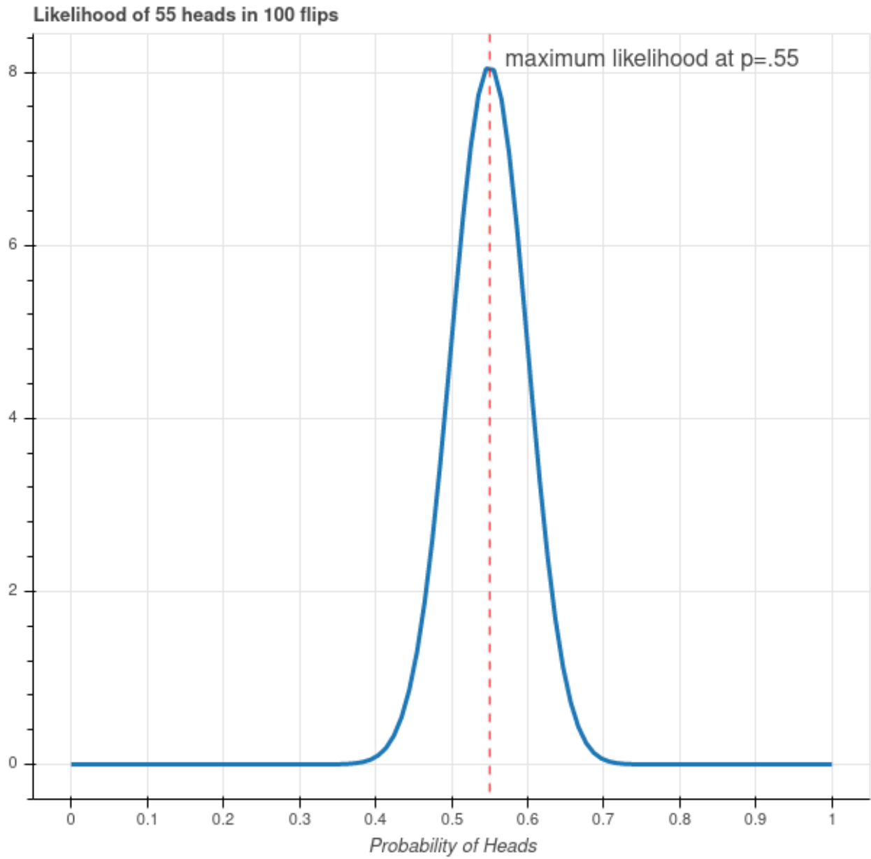
Figure 3.5: Likelihood Plot
