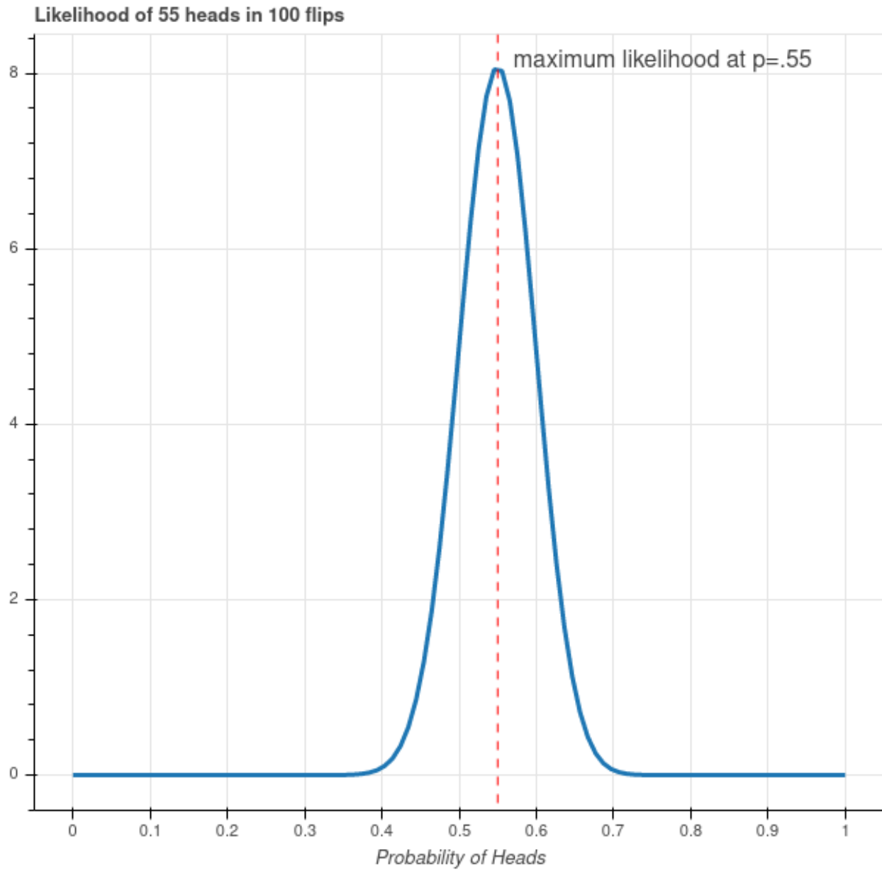
Figure 3.7: Likelihood Plot
