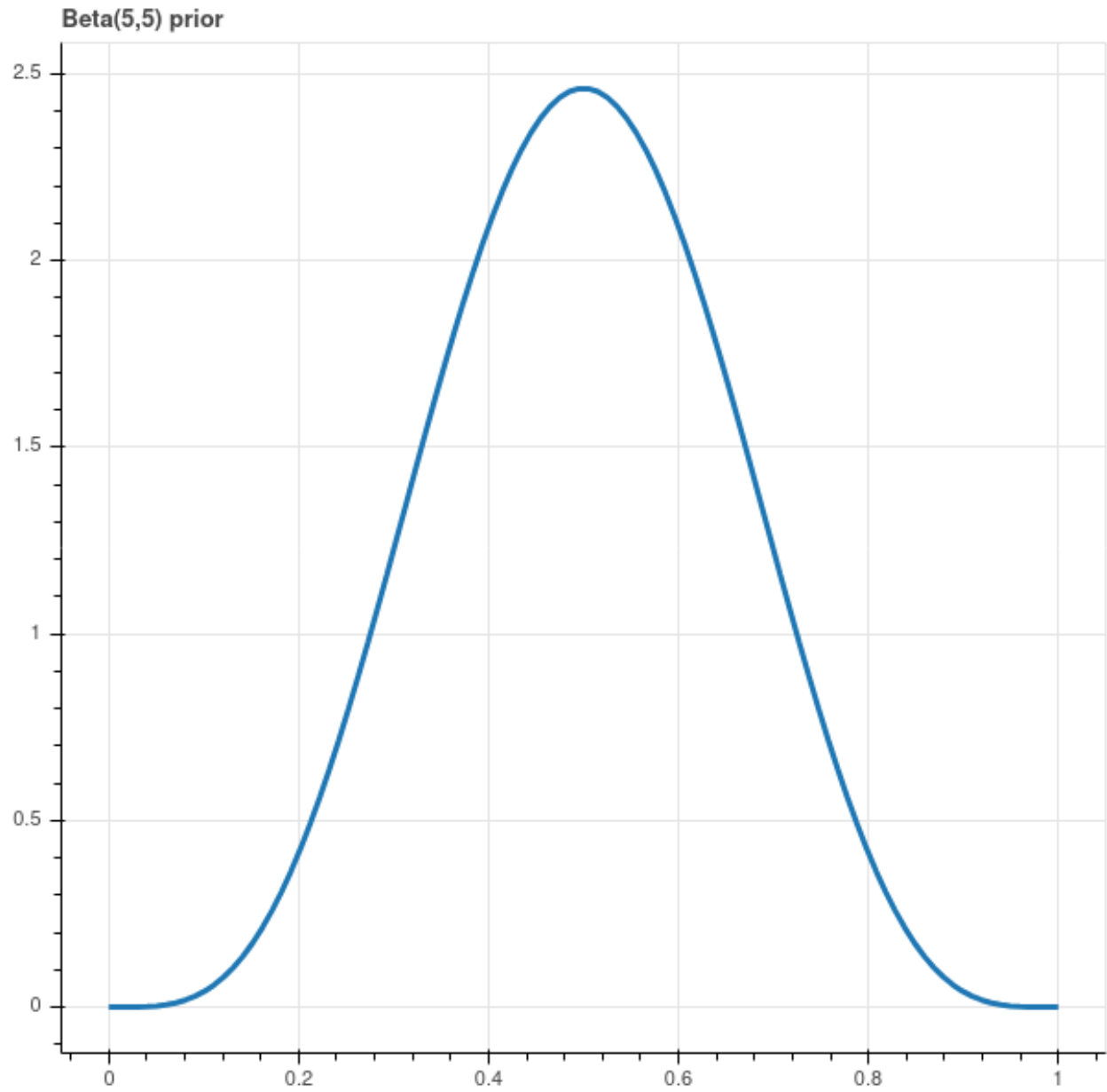
Figure 4.11: Beta(5,5) Prior
