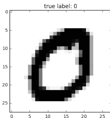
Figure 5.1: Handwritten 0
