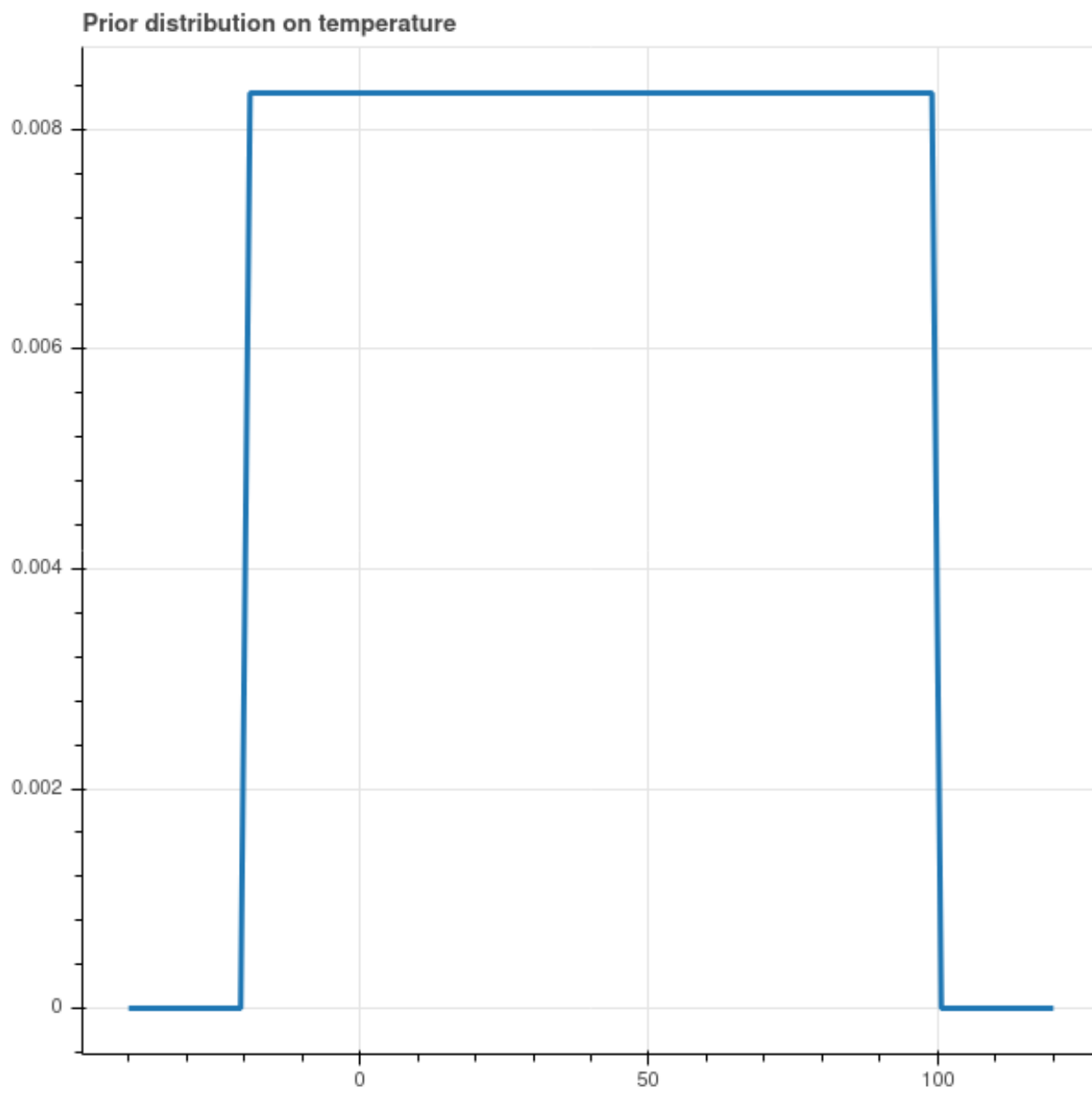
Figure 4.8: Uniform Prior
