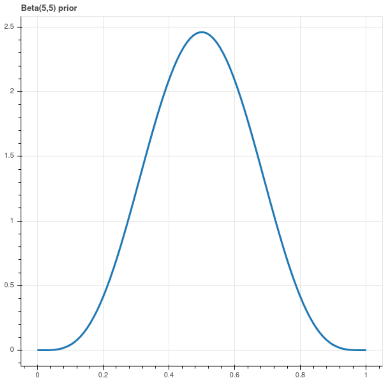
Figure 4.10: Beta(5,5) Prior
