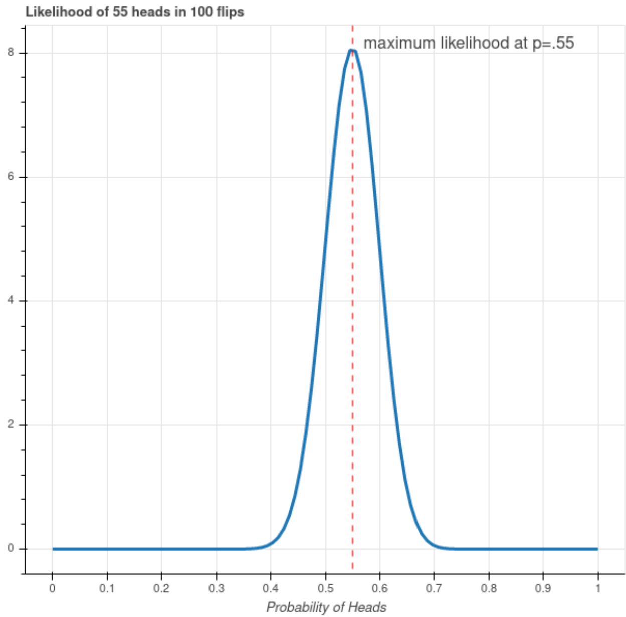
Figure 3.5: Likelihood Plot
