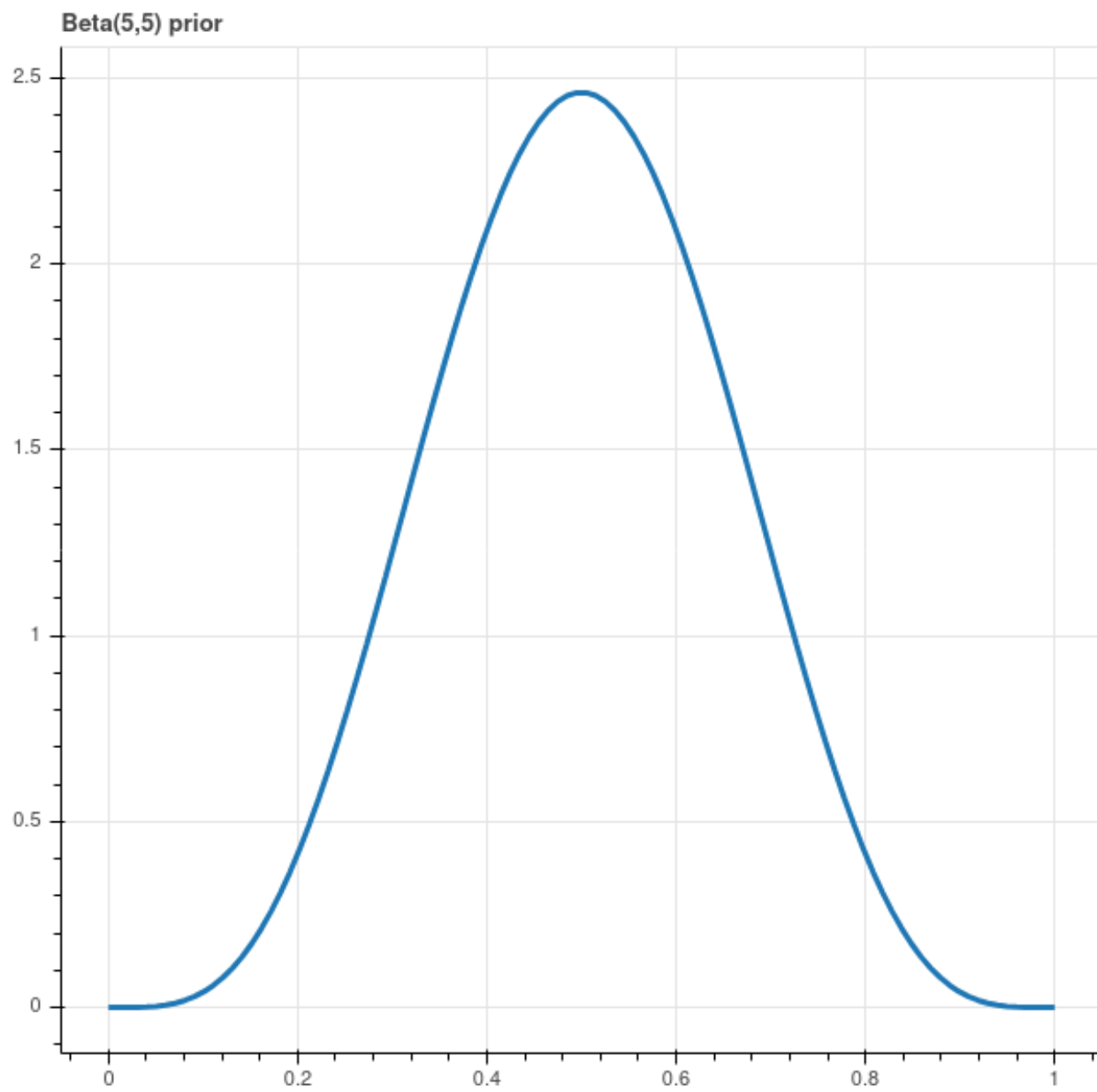
Figure 3.9: Beta(5,5) Prior
