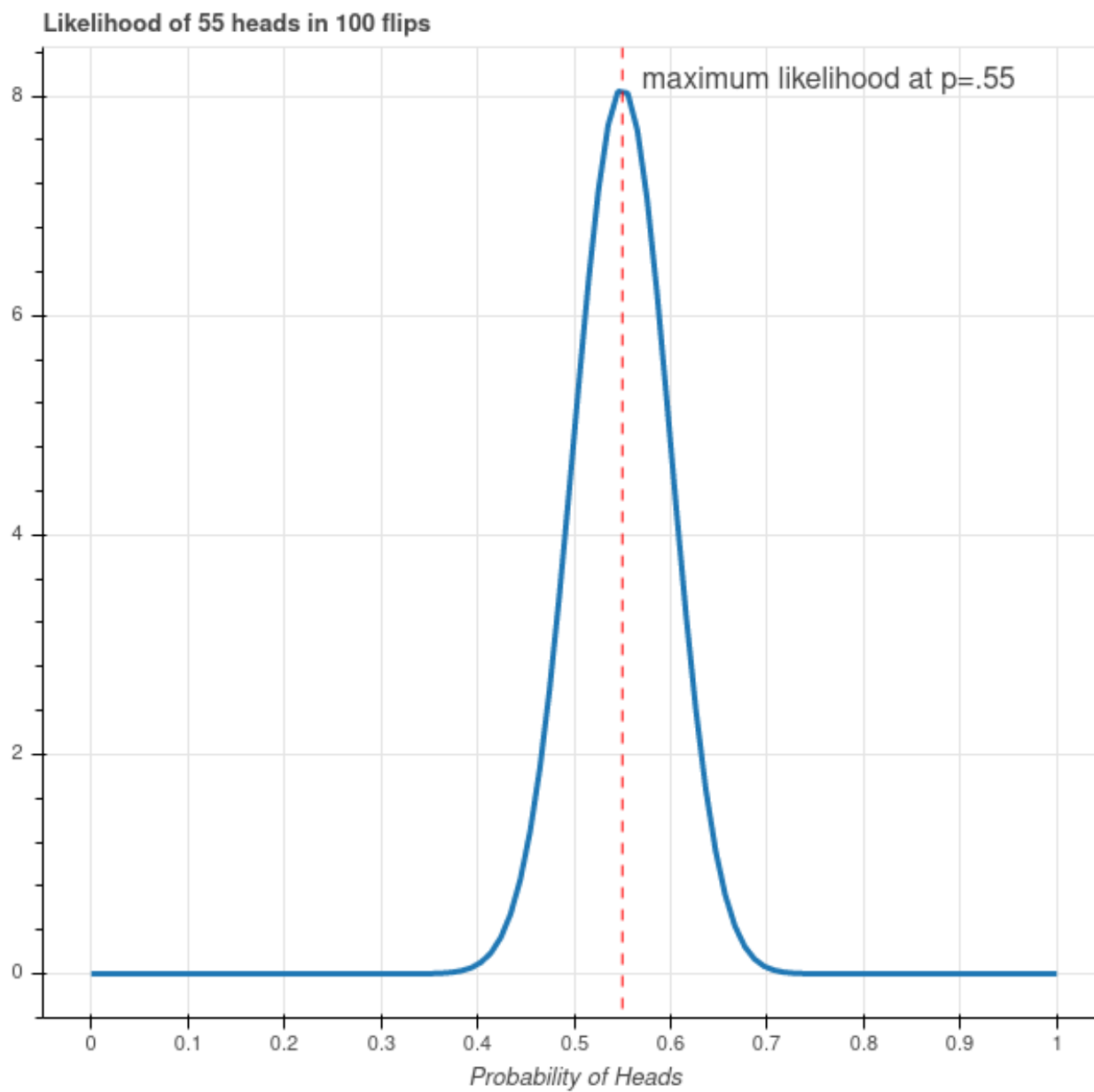
Figure 3.7: Likelihood Plot
