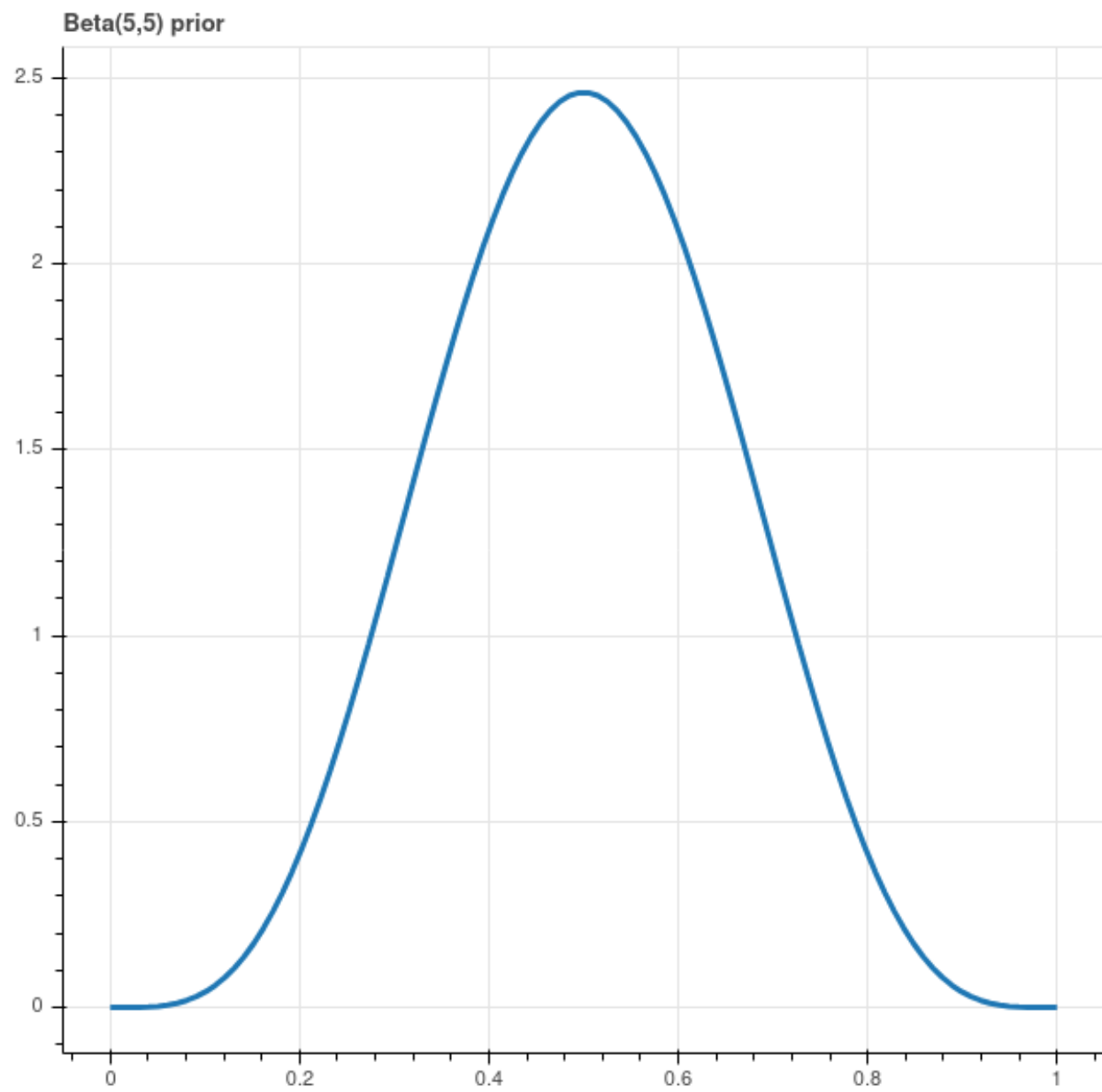
Figure 4.11: Beta(5,5) Prior
