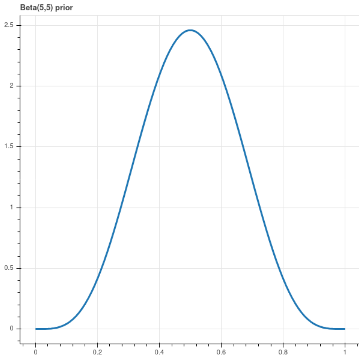
Figure 3.9: Beta(5,5) Prior
