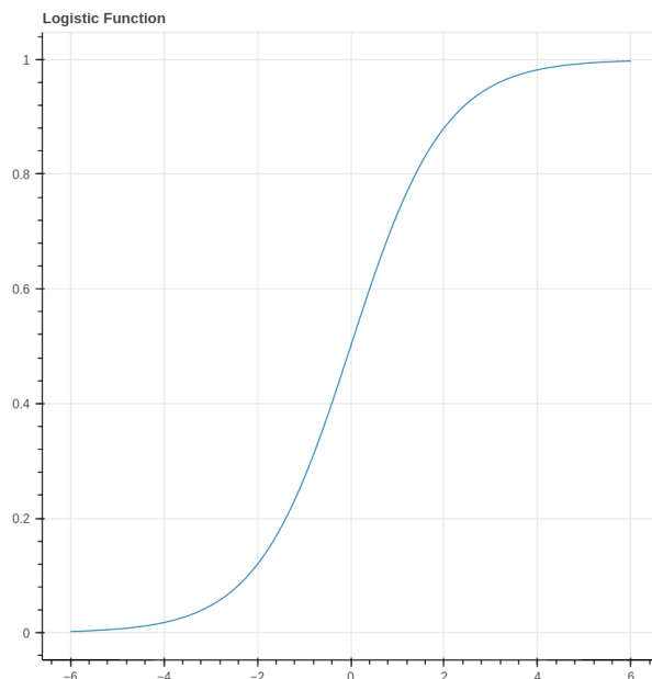
Figure 7.1: Logistic Curve
