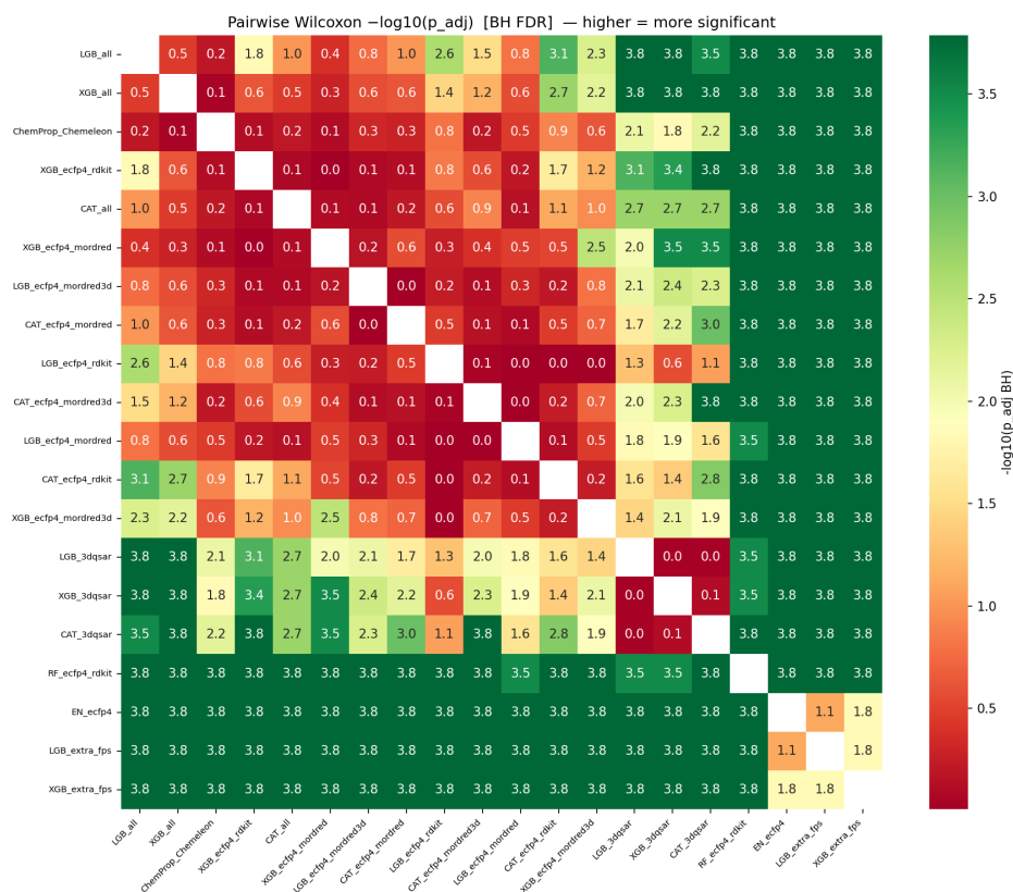
Figure 5. Heatmap of -\log_{10}(p_{\text{adj}}) [BH FDR] for all model pairs. Higher values (greener) indicate more significant differences. White cells = not significant ( p_{\text{adj}} > 0.05 ). Models ordered by mean CV RMSE (best at top-left).
