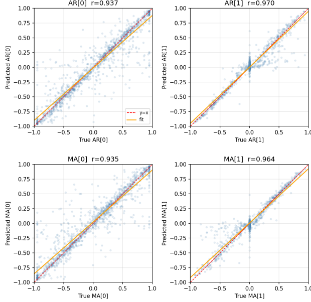
Figure 3: Full 4-coefficient scatter for the 2x2 (ARMA(2, 2)) configuration: AR_0 and AR_1 on the top row, MA_0 and MA_1 on the bottom row.
