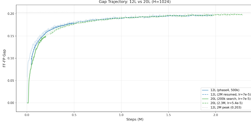
Figure 5: Contrastive gap (forecast–future minus forecast–past) over training steps for the 12L (extended to 2M steps) and 20L (extended to 2.3M steps) backbones at H = 1024 .
