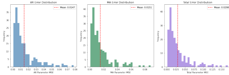
Figure 4: Per-sample MSE distributions for the recovery head on the 2x4 configuration.
