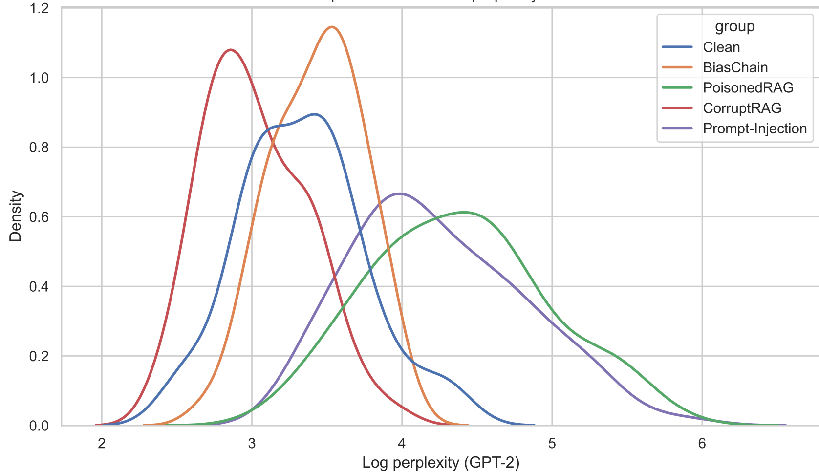
Clean and poisoned document perplexity distributions
