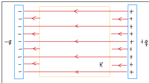
Figure 8: The surface charges on the dielectric reduce the electric field inside the dielectric.
