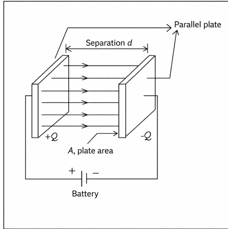
Figure 7: A basic parallel plate capacitor with charge +Q and -Q on each plate and a voltage \Delta V across them.
