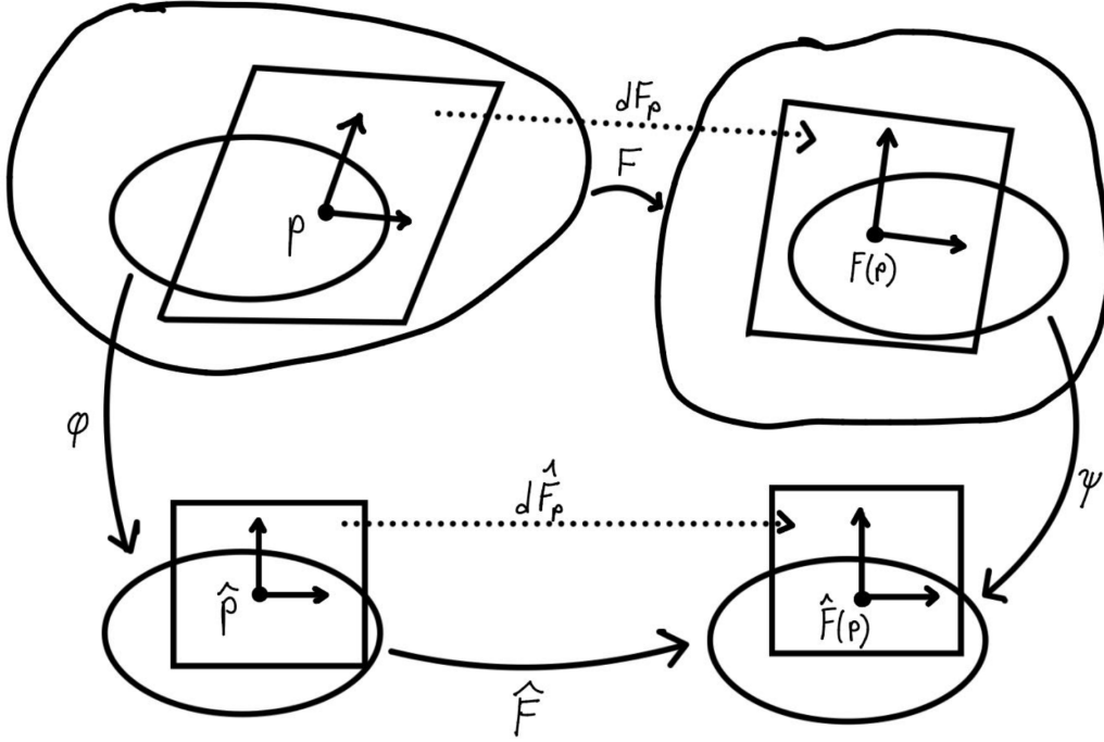
Figure 2.8: The differential dF_p relates tangent spaces of two manifolds M and N under a smooth map F : M \rightarrow N . In local coordinates (U, \varphi) and (V, \psi) , it corresponds to the ordinary Jacobian d\hat{F}_{\hat{p}} of the coordinate representation \hat{F} = \psi \circ F \circ \varphi^{-1} .
