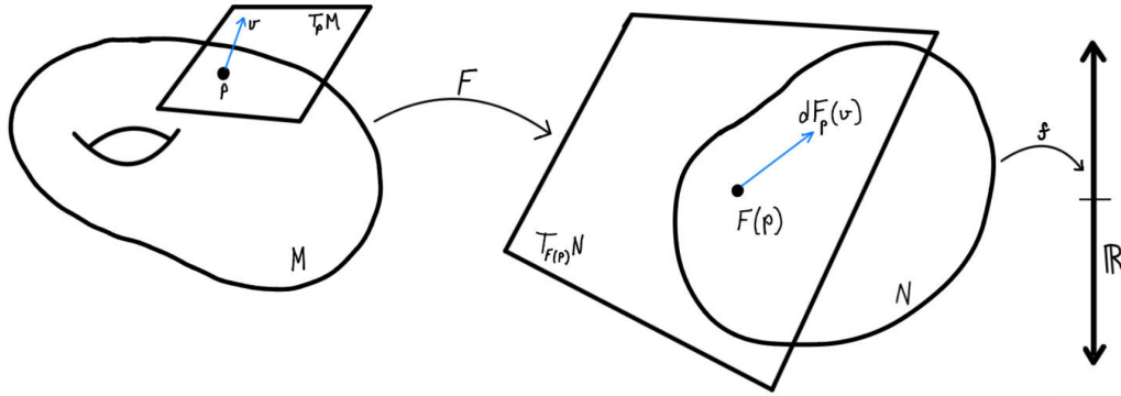
Figure 2.9: Geometric picture of the pushforward dF_p : a tangent vector v \in T_p M to a curve \gamma at p is mapped to the tangent vector dF_p(v) \in T_{F(p)} N of the image curve F \circ \gamma at F(p) . Acting on a function f : N \rightarrow \mathbb{R} , the pushforward satisfies (dF_p v)(f) = v(f \circ F) .
