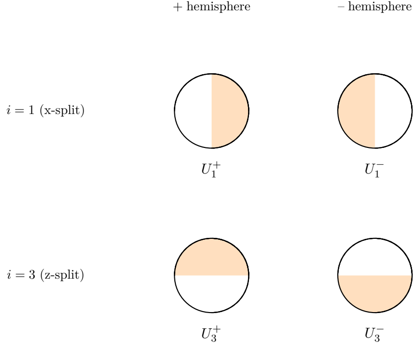
Figure 2.3: The six open hemispheres U_i^\pm = \{(x, y, z) \in S^2 : \pm x_i > 0\} for i = 1, 2, 3 (with x_1 = x , x_2 = y , x_3 = z ). Each chart f_i^\pm uses the other two Cartesian coordinates as local coordinates on U_i^\pm ; e.g. on U_3^\pm , f_3^\pm(x, y, z) = (x, y) . Shading indicates the hemisphere where the indicated coordinate is positive (left column) or negative (right column). Only the x - and z -splits ( i = 1, 3 ) are shown here for clarity—these can be drawn without obscuring the geometry. The y -split hemispheres ( i = 2 ) are analogous but lie in planes that would appear edge-on in this projection and are omitted.
