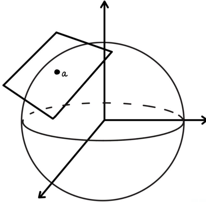
Figure 2.7: Tangent plane T_a M to a two-dimensional manifold M (the sphere) at a point a . The tangent vector \dot{\gamma}(0) represents the velocity of a curve \gamma(t) passing through a , showing how directions on M correspond to vectors in the tangent space.
