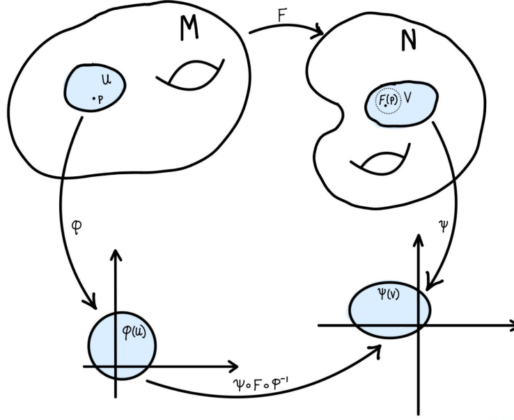
Figure 2.6: A smooth map F : M \rightarrow N between manifolds. In local coordinates, the composition \psi \circ F \circ \phi^{-1} appears as a smooth function between regions of \mathbb{R}^m and \mathbb{R}^n . This abstractly represents smooth coordinate transformations or field maps in spacetime.
