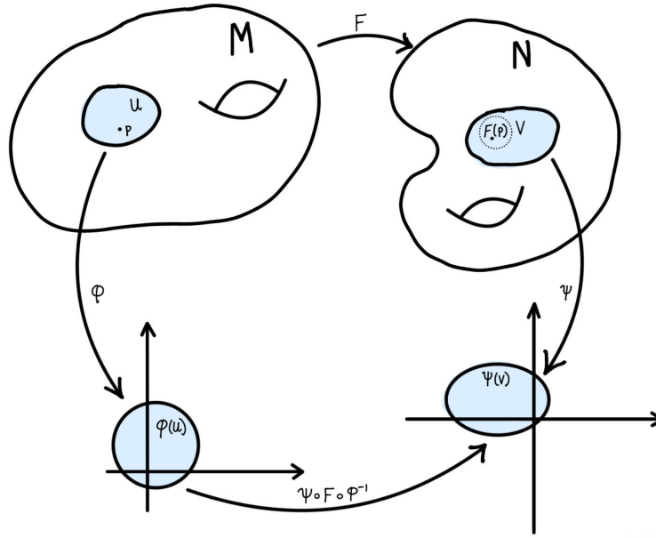
Figure 1.6: A smooth map F : M \rightarrow N between manifolds. In local coordinates, the composition \psi \circ F \circ \phi^{-1} is an ordinary smooth map between regions of \mathbb{R}^m and \mathbb{R}^n .
