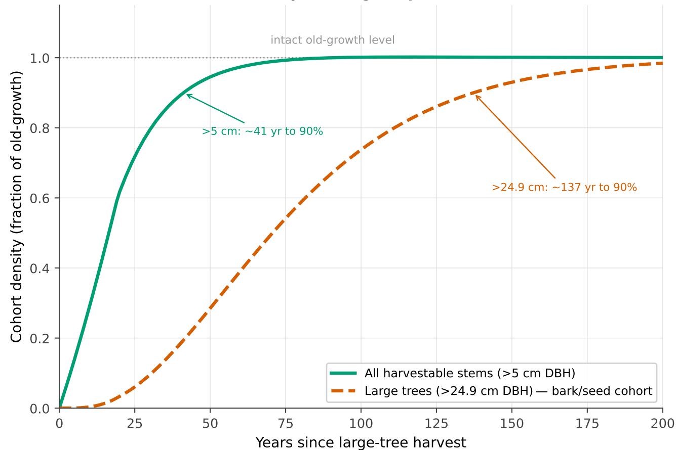
(a) Post-harvest recovery (Busing & Spies 1995 matrix, \lambda = 1.02 )
