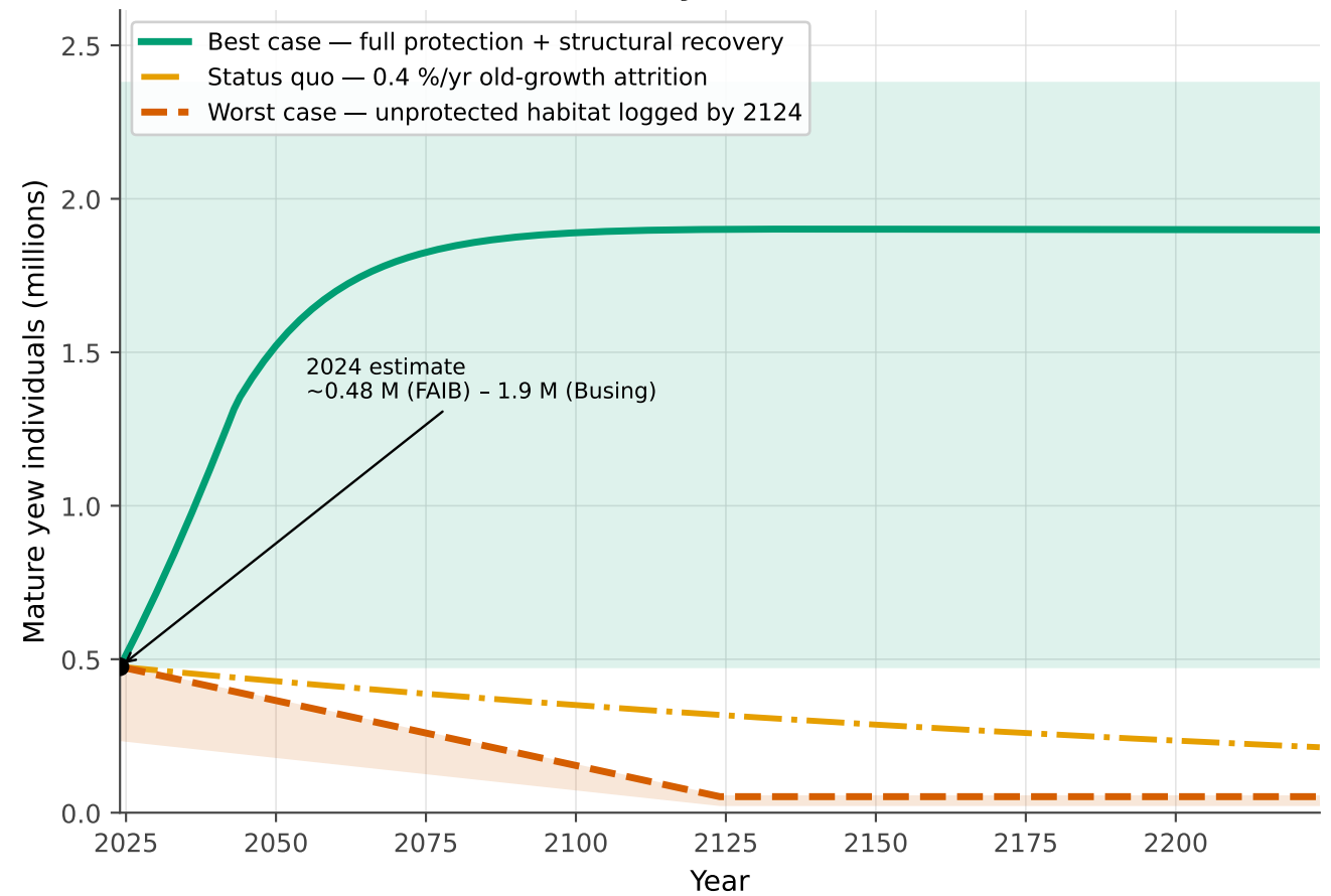
(b) Province-scale mature yew (DBH \geq 10 cm), 2024-2224
