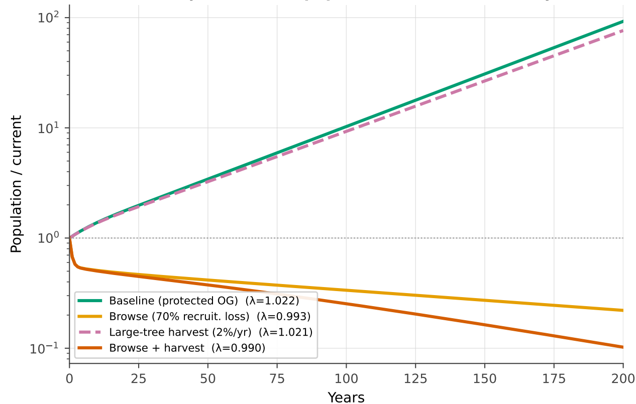
(a) Projected stand population (relative to today)
