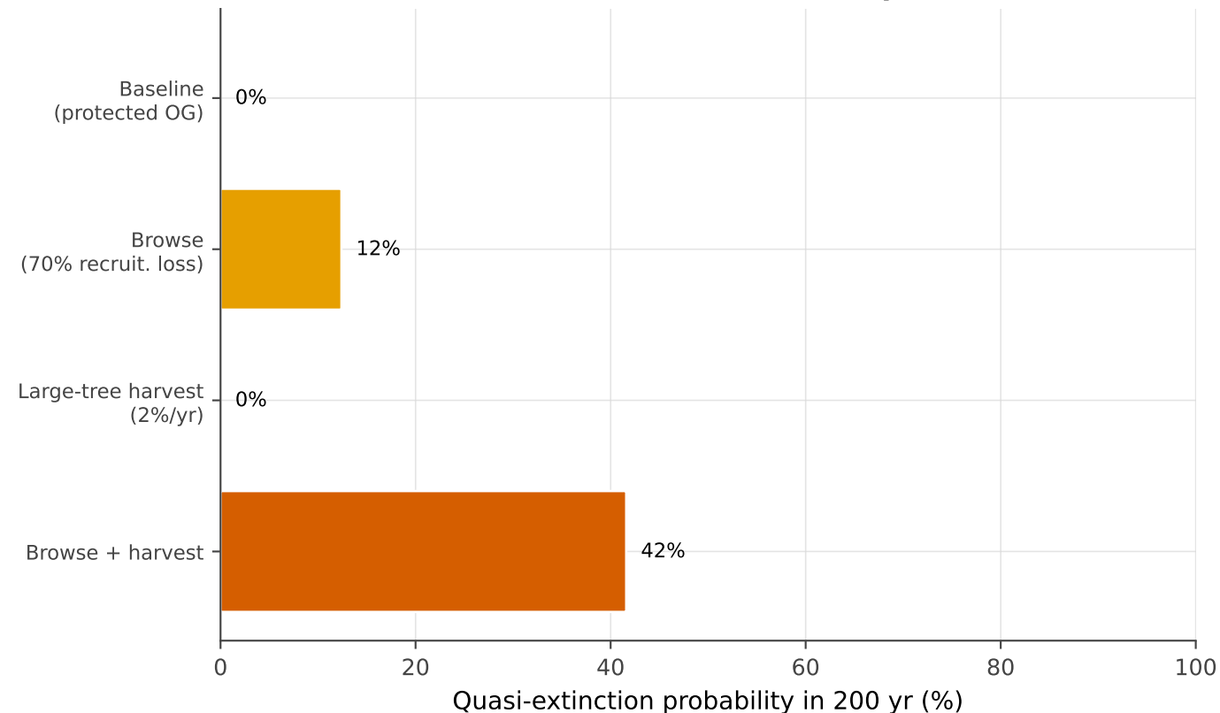
(b) Quasi-extinction probability ( <10\% of current, 500 stochastic reps, CV=0.15 )
