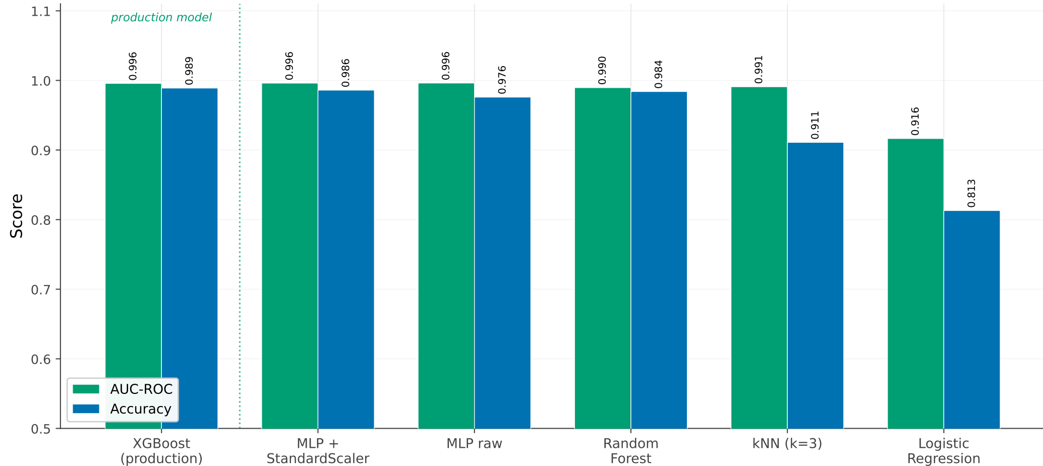
Classifier Performance on 64-band AlphaEarth Embeddings (held-out validation set; y-axis truncated at 0.5)
