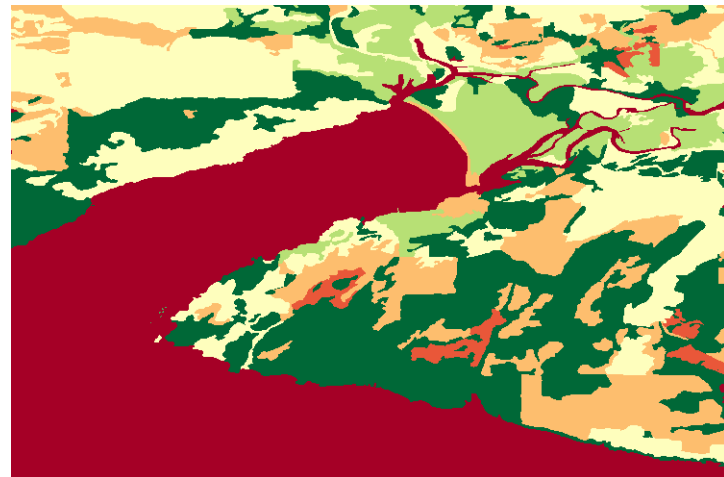
Logging status
