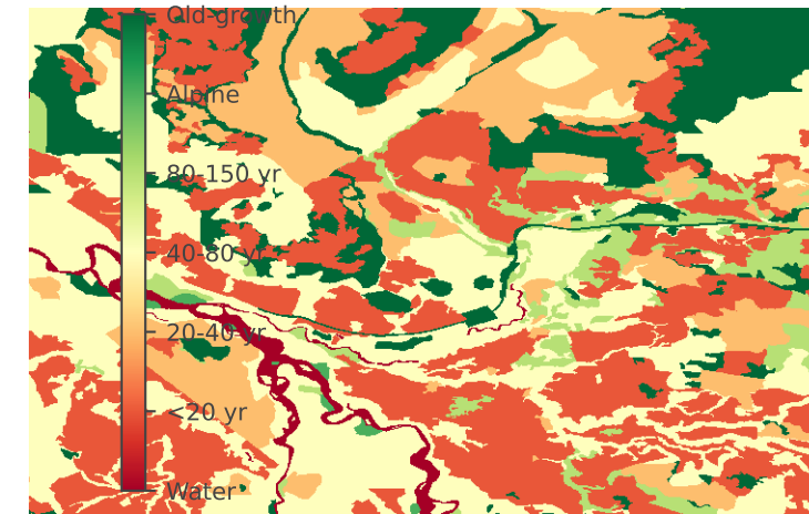
Logging status
