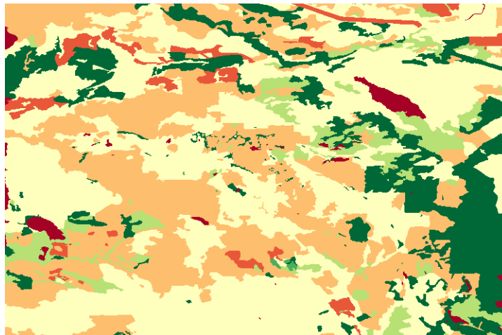
Logging status
