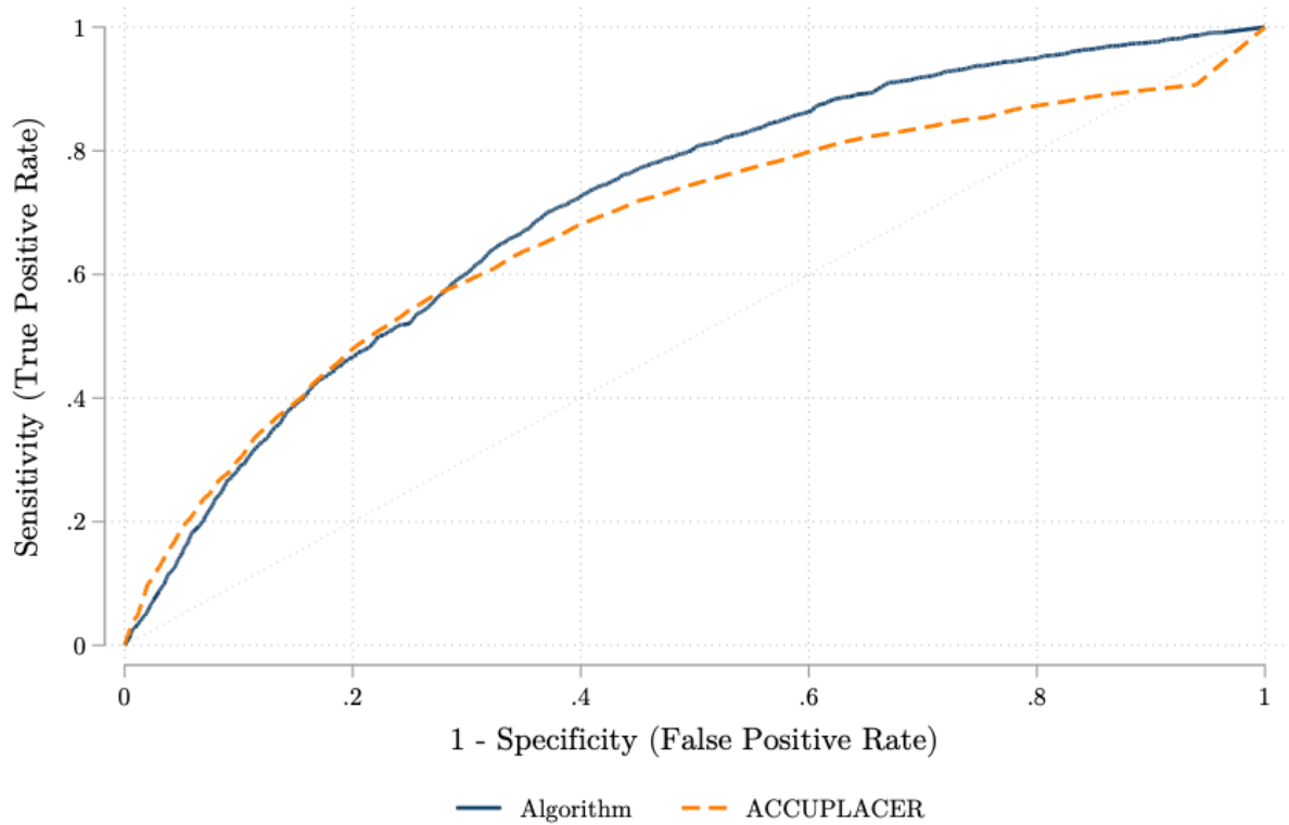
Figure A.1. ROC Curves: Math Placement
