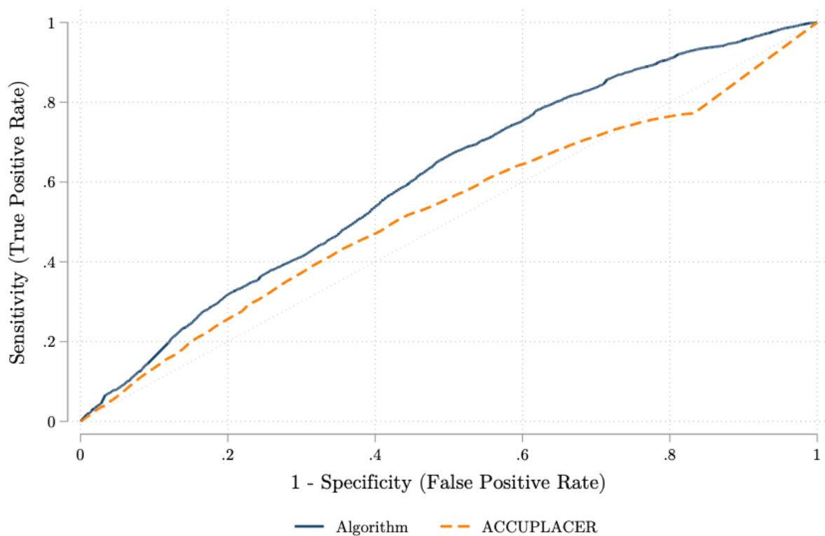
Figure A.2. ROC Curves: English Placement
