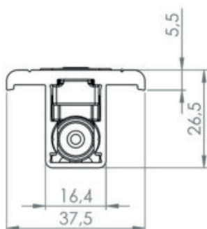
Dwarsdoorsnede NX-3809 RAAM
