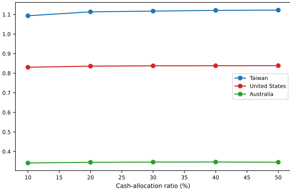
Full-sample Sortino ratio
