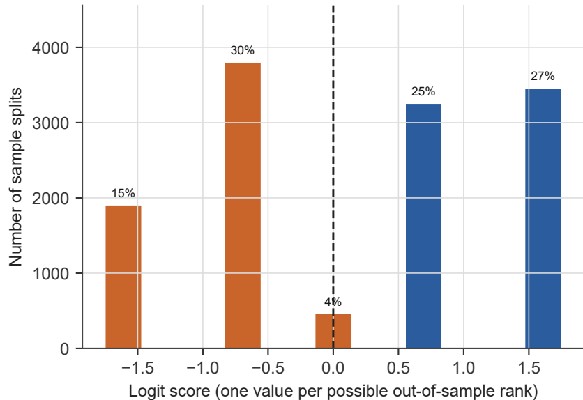
(a) Taiwan (0050): probability of backtest overfitting = 47.9%
