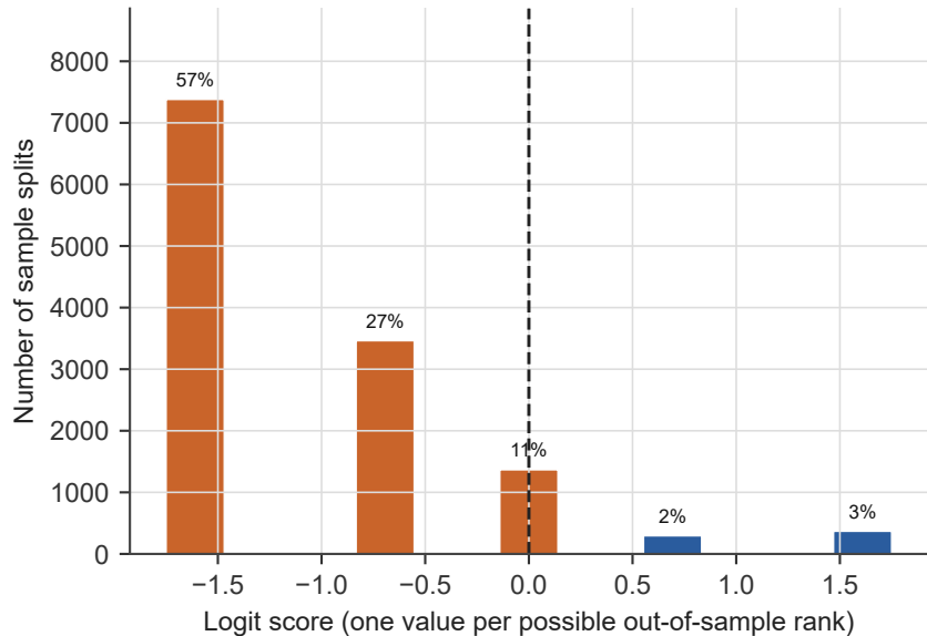
(b) United States (SPY): probability of backtest overfitting = 94.9%
