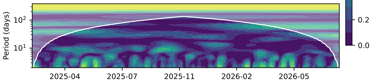
sUSDS vs. FANG: wavelet coherence
