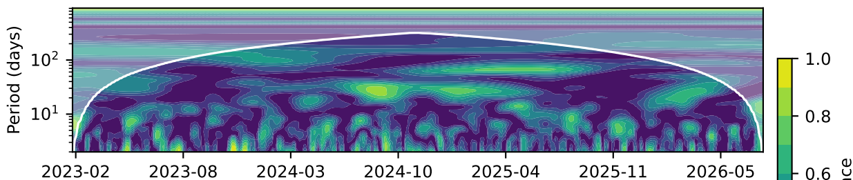
OUSG vs. FANG: wavelet coherence
