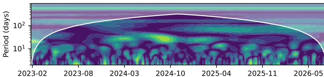
OUSG vs. SOXX: wavelet coherence
